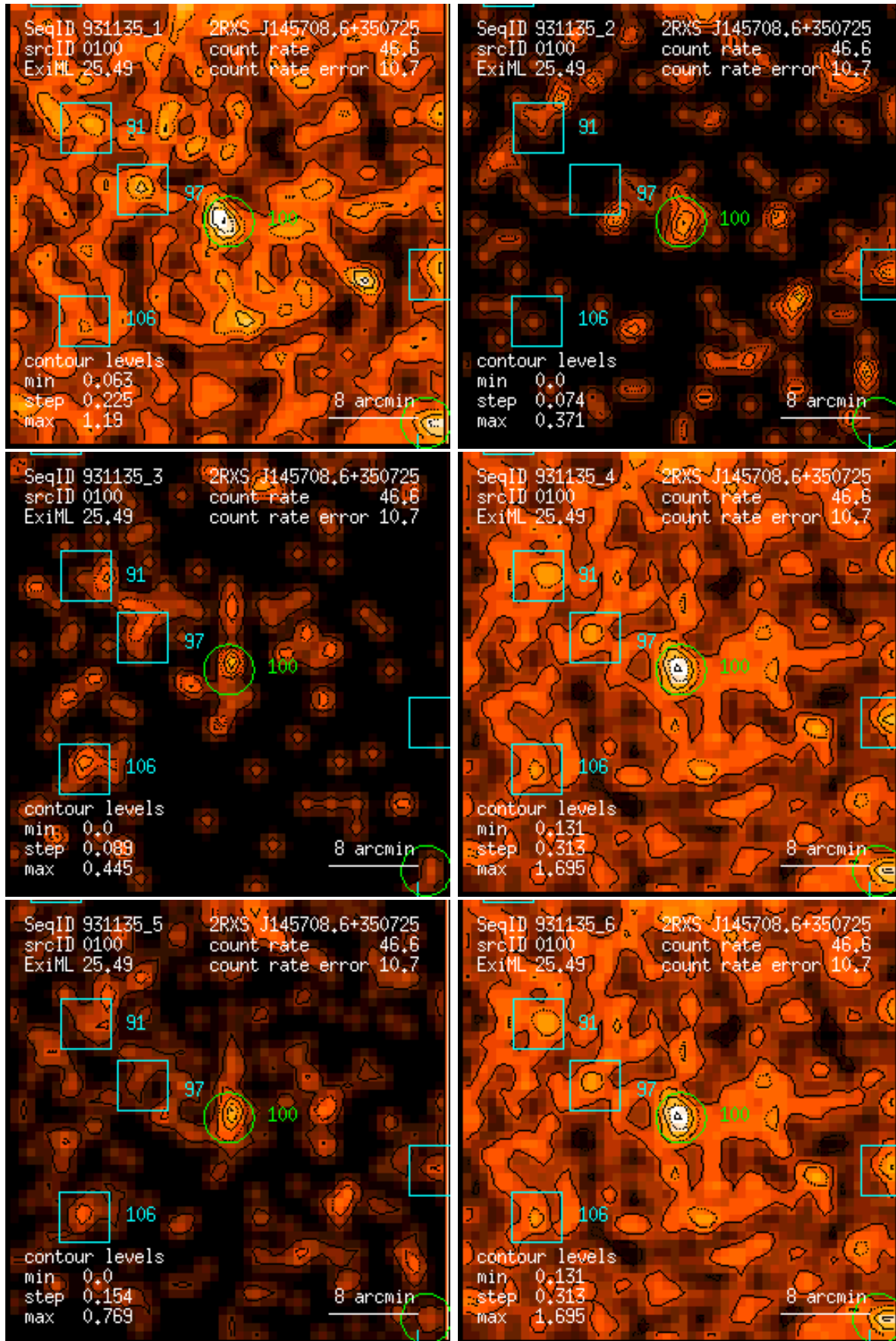
Figure 100: RASS 931135: detection 0100: band rate images, Gaussian filter: (1) PSPC channels 11 – 41, (2) 52 – 90, (3) 91 – 201, (4) 11 – 235, (5) 52 – 201, (6) 11 – 201. Broad band rates in counts/ks. Band rate contour levels in counts/ks/arcmin 2 .
