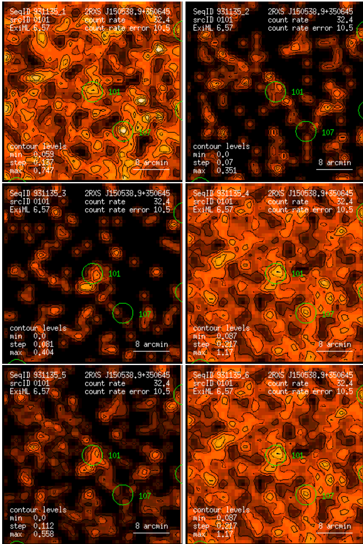
Figure 101: RASS 931135: detection 0101: band rate images, Gaussian filter: (1) PSPC channels 11 – 41, (2) 52 – 90, (3) 91 – 201, (4) 11 – 235, (5) 52 – 201, (6) 11 – 201. Broad band rates in counts/ks. Band rate contour levels in counts/ks/arcmin 2 .
