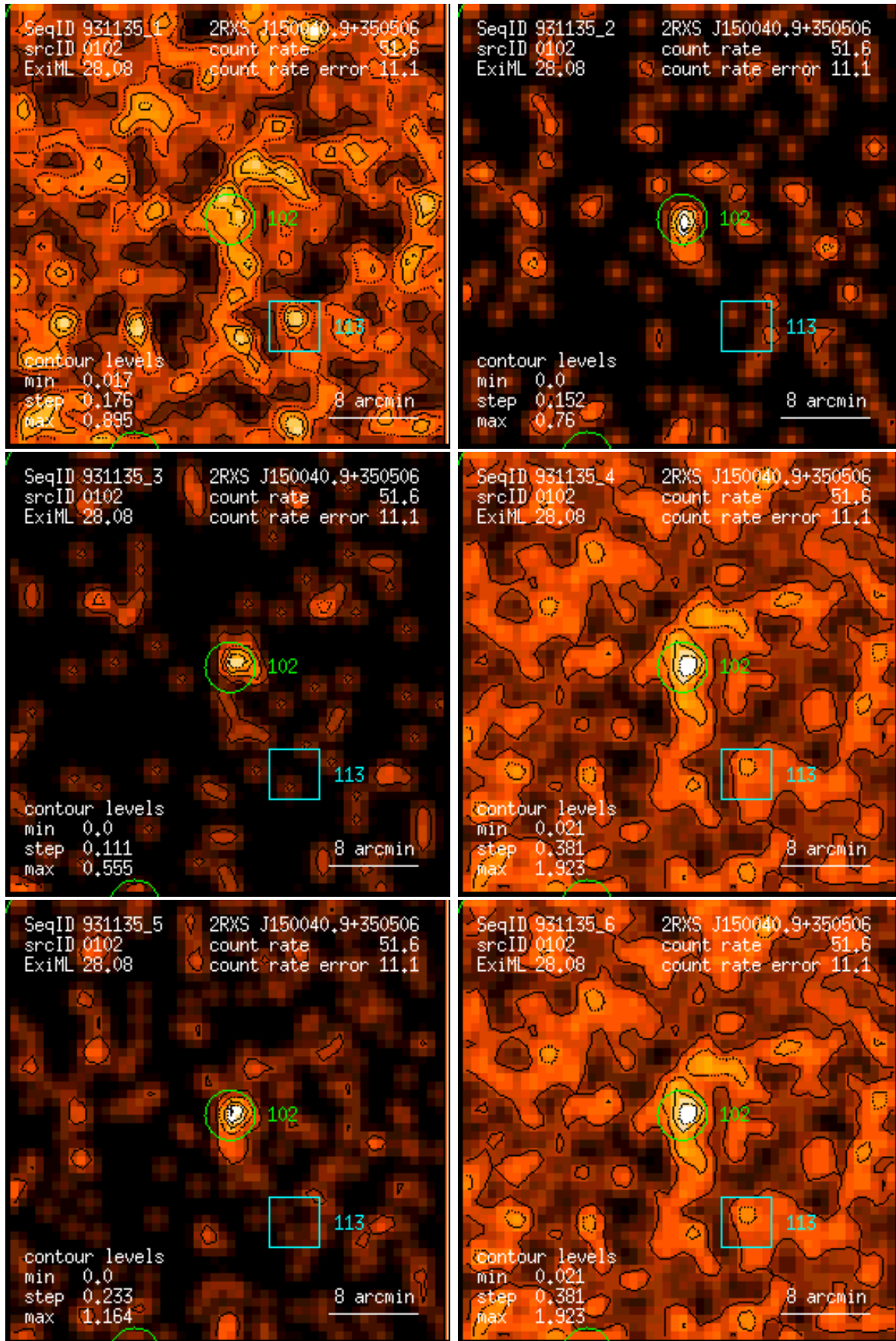
Figure 102: RASS 931135: detection 0102: band rate images, Gaussian filter: (1) PSPC channels 11 – 41, (2) 52 – 90, (3) 91 – 201, (4) 11 – 235, (5) 52 – 201, (6) 11 – 201. Broad band rates in counts/ks. Band rate contour levels in counts/ks/arcmin 2 .
