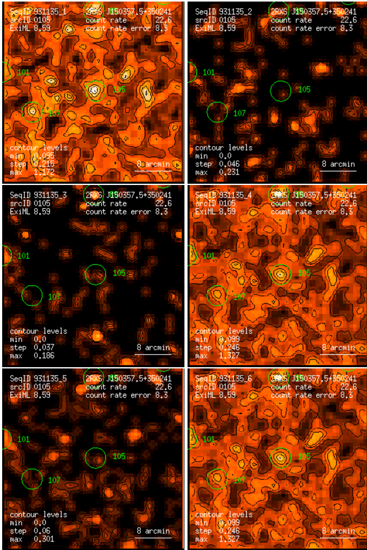
Figure 105: RASS 931135: detection 0105: band rate images, Gaussian filter: (1) PSPC channels 11 – 41, (2) 52 – 90, (3) 91 – 201, (4) 11 – 235, (5) 52 – 201, (6) 11 – 201. Broad band rates in counts/ks. Band rate contour levels in counts/ks/arcmin 2 .
