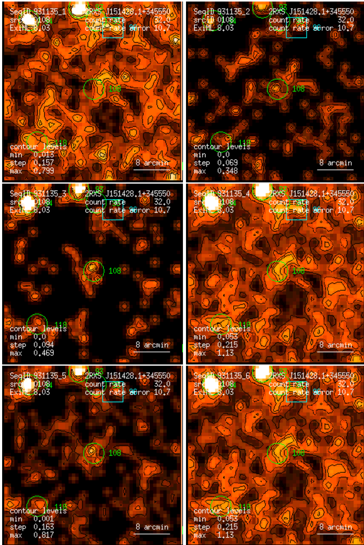
Figure 108: RASS 931135: detection 0108: band rate images, Gaussian filter: (1) PSPC channels 11 – 41, (2) 52 – 90, (3) 91 – 201, (4) 11 – 235, (5) 52 – 201, (6) 11 – 201. Broad band rates in counts/ks. Band rate contour levels in counts/ks/arcmin 2 .
