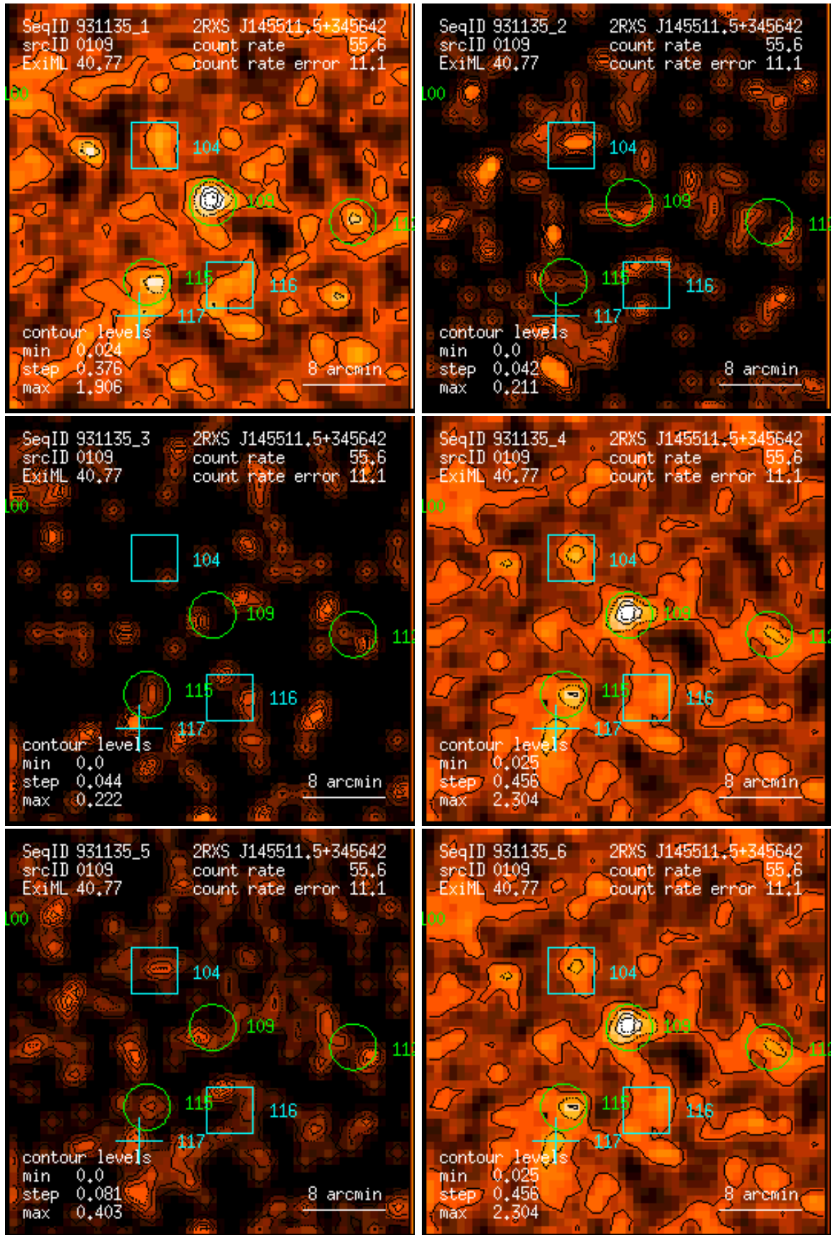
Figure 109: RASS 931135: detection 0109: band rate images, Gaussian filter: (1) PSPC channels 11 – 41, (2) 52 – 90, (3) 91 – 201, (4) 11 – 235, (5) 52 – 201, (6) 11 – 201. Broad band rates in counts/ks. Band rate contour levels in counts/ks/arcmin 2 .
