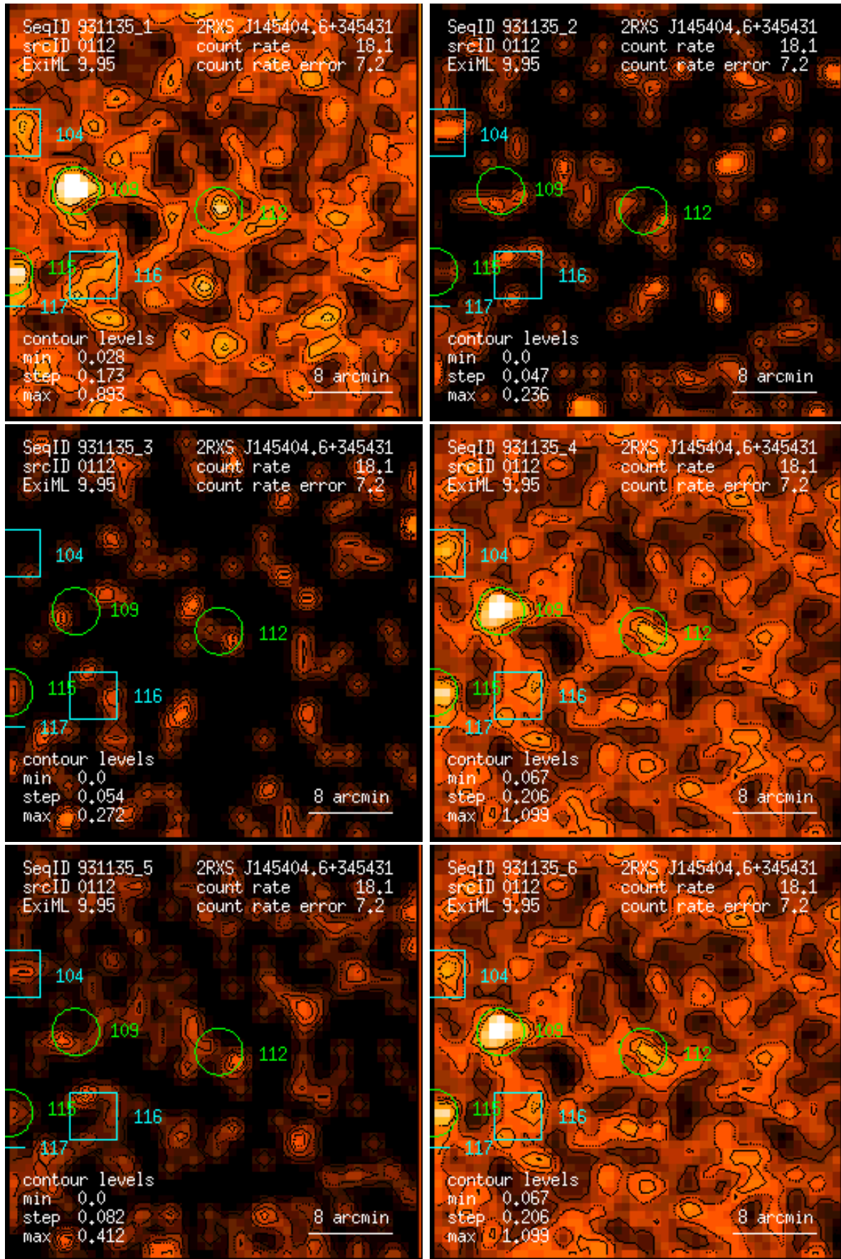
Figure 112: RASS 931135: detection 0112: band rate images, Gaussian filter: (1) PSPC channels 11 – 41, (2) 52 – 90, (3) 91 – 201, (4) 11 – 235, (5) 52 – 201, (6) 11 – 201. Broad band rates in counts/ks. Band rate contour levels in counts/ks/arcmin 2 .
