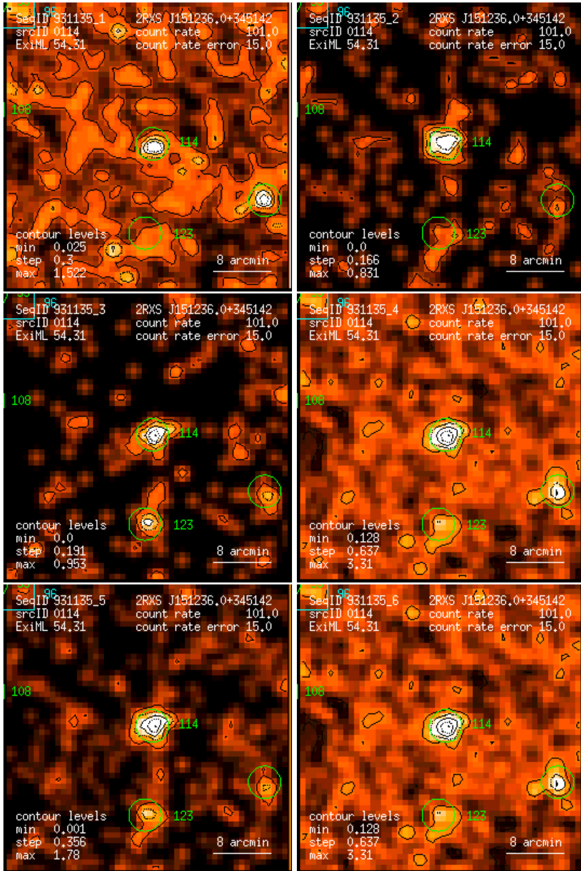
Figure 114: RASS 931135: detection 0114: band rate images, Gaussian filter: (1) PSPC channels 11 – 41, (2) 52 – 90, (3) 91 – 201, (4) 11 – 235, (5) 52 – 201, (6) 11 – 201. Broad band rates in counts/ks. Band rate contour levels in counts/ks/arcmin 2 .
