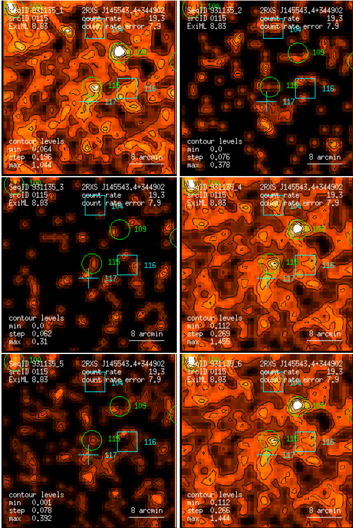
Figure 115: RASS 931135: detection 0115: band rate images, Gaussian filter: (1) PSPC channels 11 – 41, (2) 52 – 90, (3) 91 – 201, (4) 11 – 235, (5) 52 – 201, (6) 11 – 201. Broad band rates in counts/ks. Band rate contour levels in counts/ks/arcmin 2 .
