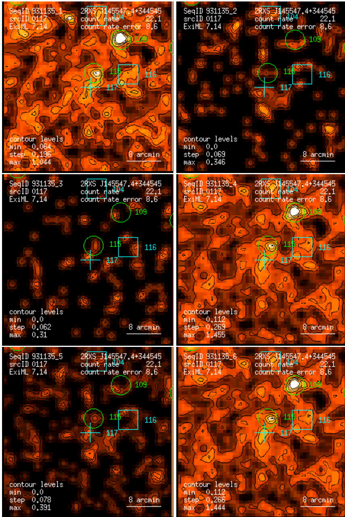
Figure 117: RASS 931135: detection 0117: band rate images, Gaussian filter: (1) PSPC channels 11 – 41, (2) 52 – 90, (3) 91 – 201, (4) 11 – 235, (5) 52 – 201, (6) 11 – 201. Broad band rates in counts/ks. Band rate contour levels in counts/ks/arcmin 2 .
