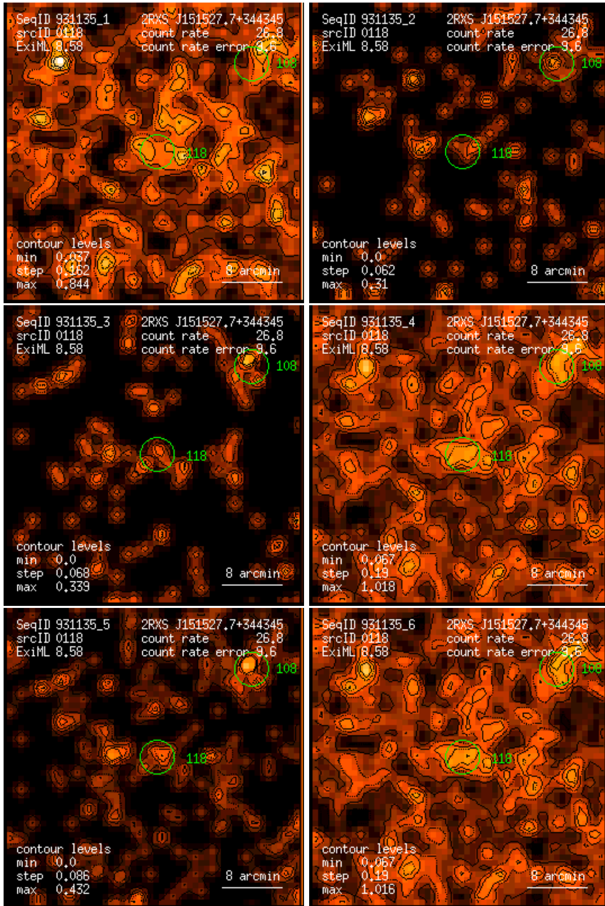
Figure 118: RASS 931135: detection 0118: band rate images, Gaussian filter: (1) PSPC channels 11 – 41, (2) 52 – 90, (3) 91 – 201, (4) 11 – 235, (5) 52 – 201, (6) 11 – 201. Broad band rates in counts/ks. Band rate contour levels in counts/ks/arcmin 2 .
