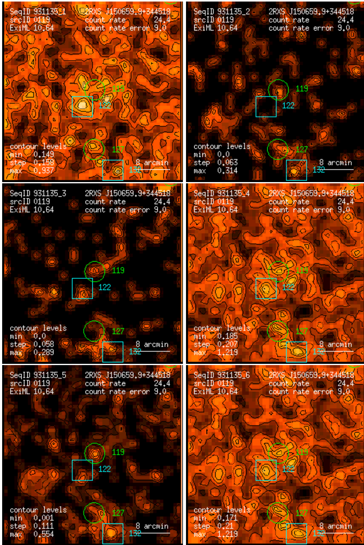
Figure 119: RASS 931135: detection 0119: band rate images, Gaussian filter: (1) PSPC channels 11 – 41, (2) 52 – 90, (3) 91 – 201, (4) 11 – 235, (5) 52 – 201, (6) 11 – 201. Broad band rates in counts/ks. Band rate contour levels in counts/ks/arcmin 2 .
