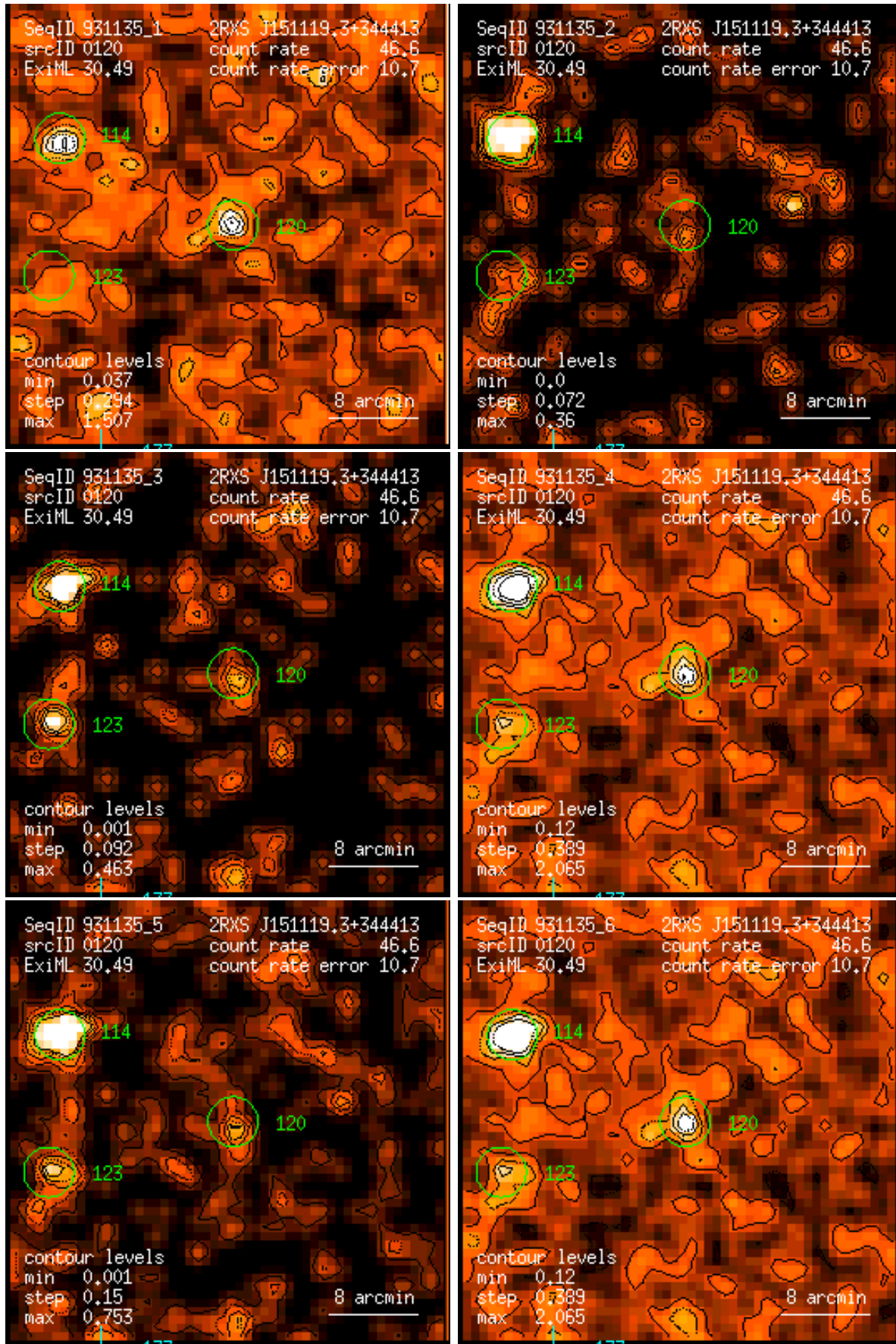
Figure 120: RASS 931135: detection 0120: band rate images, Gaussian filter: (1) PSPC channels 11 – 41, (2) 52 – 90, (3) 91 – 201, (4) 11 – 235, (5) 52 – 201, (6) 11 – 201. Broad band rates in counts/ks. Band rate contour levels in counts/ks/arcmin 2 .
