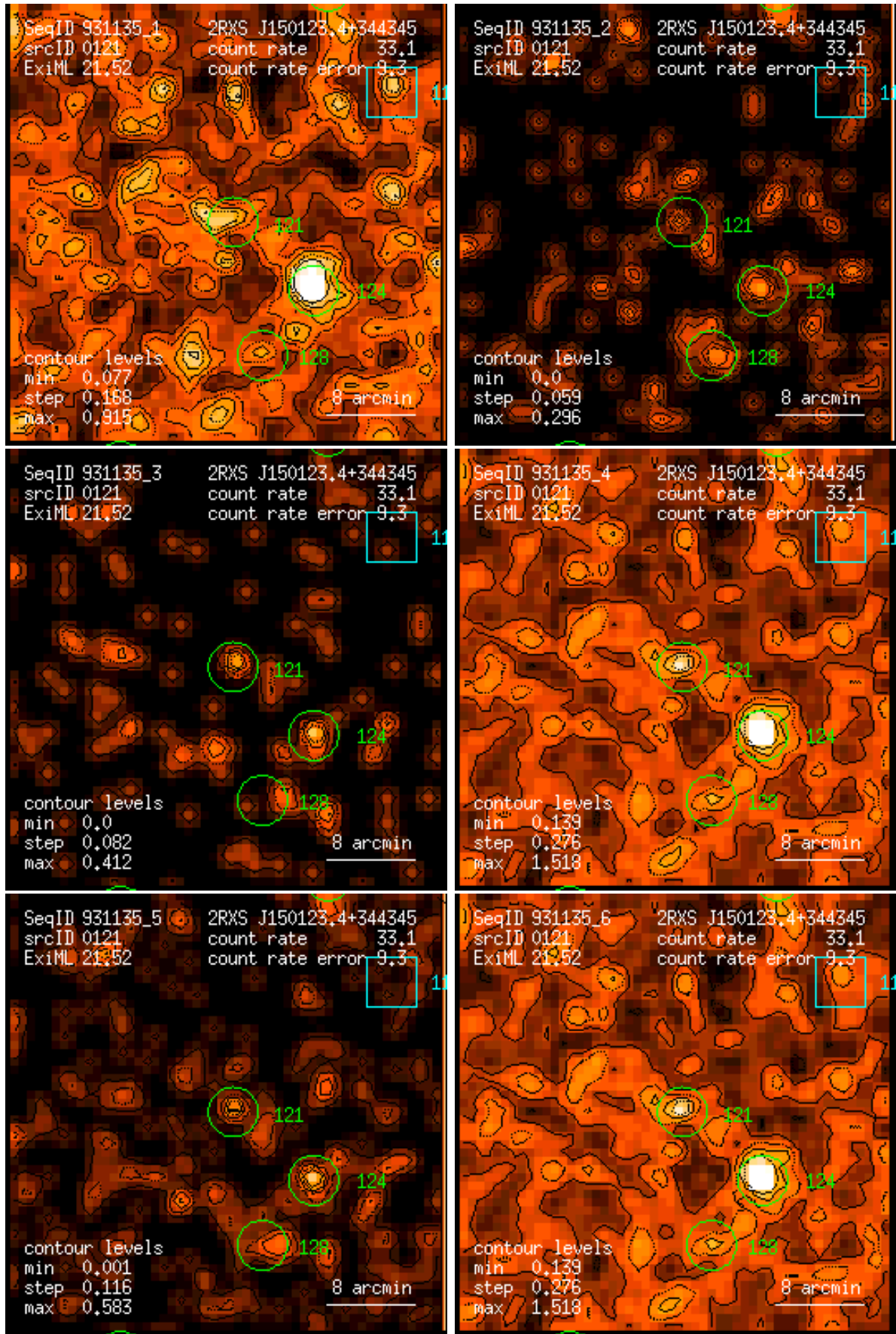
Figure 121: RASS 931135: detection 0121: band rate images, Gaussian filter: (1) PSPC channels 11 – 41, (2) 52 – 90, (3) 91 – 201, (4) 11 – 235, (5) 52 – 201, (6) 11 – 201. Broad band rates in counts/ks. Band rate contour levels in counts/ks/arcmin 2 .
