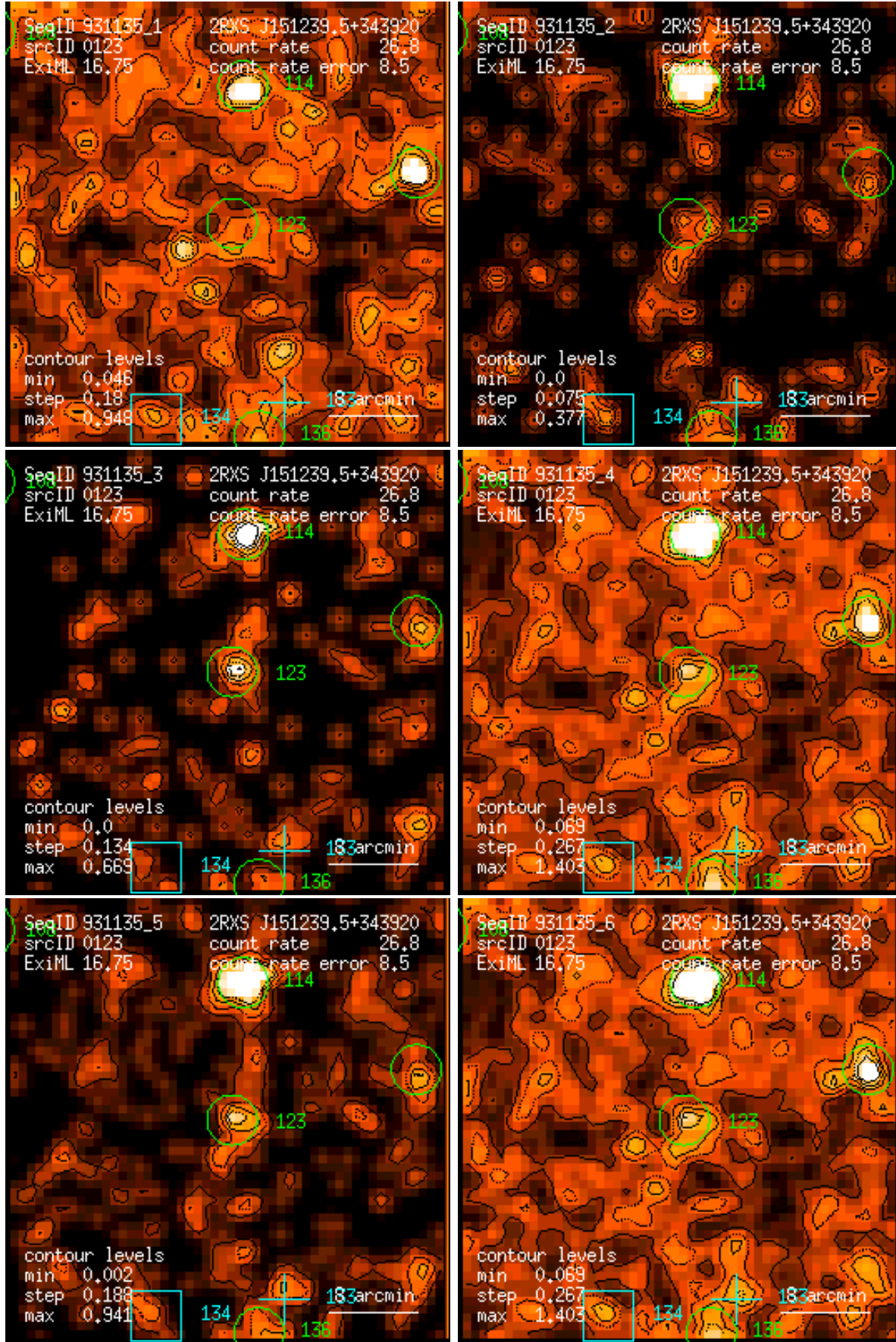
Figure 123: RASS 931135: detection 0123: band rate images, Gaussian filter: (1) PSPC channels 11 – 41, (2) 52 – 90, (3) 91 – 201, (4) 11 – 235, (5) 52 – 201, (6) 11 – 201. Broad band rates in counts/ks. Band rate contour levels in counts/ks/arcmin 2 .
