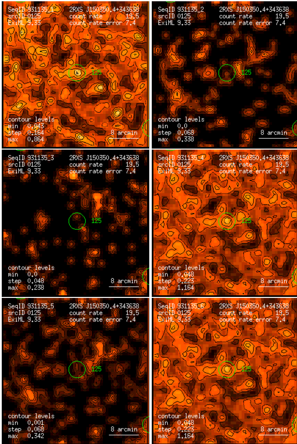
Figure 125: RASS 931135: detection 0125: band rate images, Gaussian filter: (1) PSPC channels 11 – 41, (2) 52 – 90, (3) 91 – 201, (4) 11 – 235, (5) 52 – 201, (6) 11 – 201. Broad band rates in counts/ks. Band rate contour levels in counts/ks/arcmin 2 .
