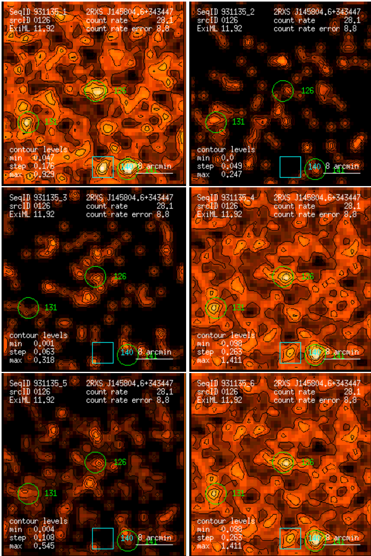
Figure 126: RASS 931135: detection 0126: band rate images, Gaussian filter: (1) PSPC channels 11 – 41, (2) 52 – 90, (3) 91 – 201, (4) 11 – 235, (5) 52 – 201, (6) 11 – 201. Broad band rates in counts/ks. Band rate contour levels in counts/ks/arcmin 2 .
