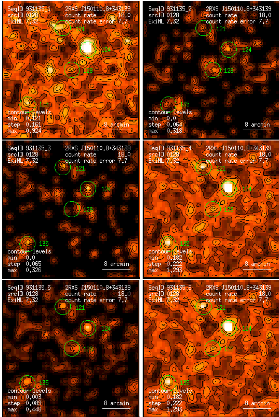
Figure 128: RASS 931135: detection 0128: band rate images, Gaussian filter: (1) PSPC channels 11 – 41, (2) 52 – 90, (3) 91 – 201, (4) 11 – 235, (5) 52 – 201, (6) 11 – 201. Broad band rates in counts/ks. Band rate contour levels in counts/ks/arcmin 2 .
