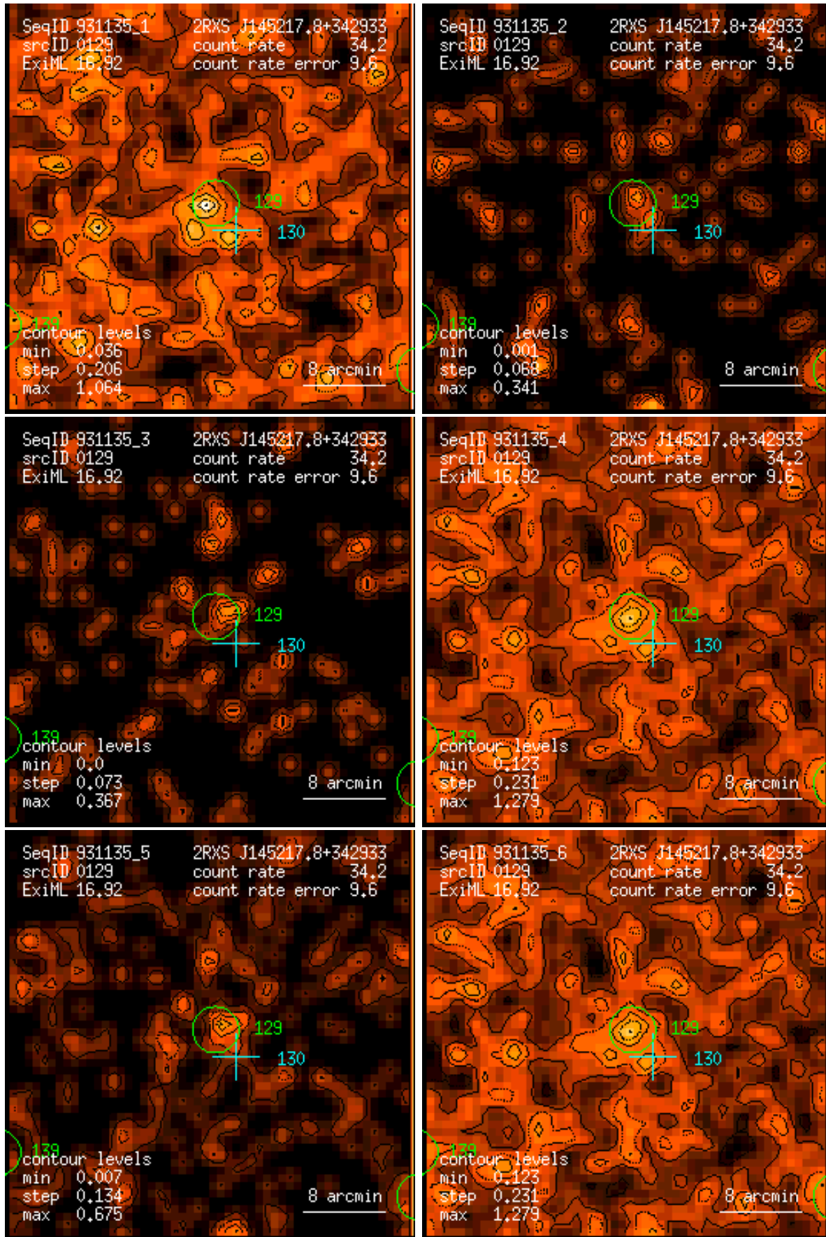
Figure 129: RASS 931135: detection 0129: band rate images, Gaussian filter: (1) PSPC channels 11 – 41, (2) 52 – 90, (3) 91 – 201, (4) 11 – 235, (5) 52 – 201, (6) 11 – 201. Broad band rates in counts/ks. Band rate contour levels in counts/ks/arcmin 2 .
