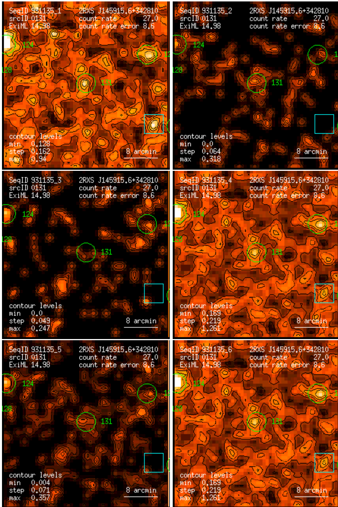
Figure 131: RASS 931135: detection 0131: band rate images, Gaussian filter: (1) PSPC channels 11 – 41, (2) 52 – 90, (3) 91 – 201, (4) 11 – 235, (5) 52 – 201, (6) 11 – 201. Broad band rates in counts/ks. Band rate contour levels in counts/ks/arcmin 2 .
