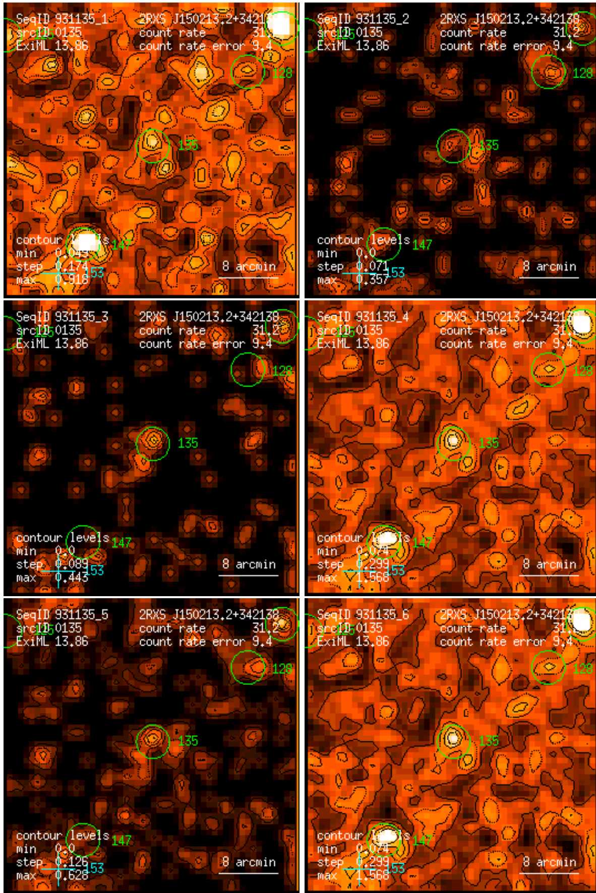
Figure 135: RASS 931135: detection 0135: band rate images, Gaussian filter: (1) PSPC channels 11 – 41, (2) 52 – 90, (3) 91 – 201, (4) 11 – 235, (5) 52 – 201, (6) 11 – 201. Broad band rates in counts/ks. Band rate contour levels in counts/ks/arcmin 2 .
