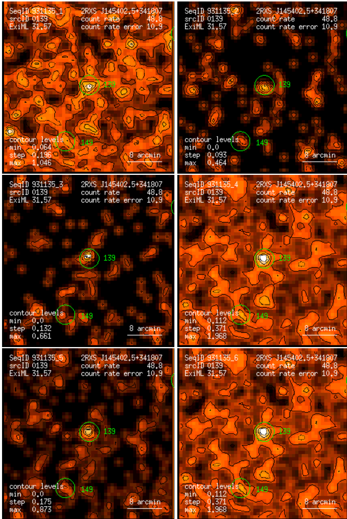
Figure 139: RASS 931135: detection 0139: band rate images, Gaussian filter: (1) PSPC channels 11 – 41, (2) 52 – 90, (3) 91 – 201, (4) 11 – 235, (5) 52 – 201, (6) 11 – 201. Broad band rates in counts/ks. Band rate contour levels in counts/ks/arcmin 2 .
