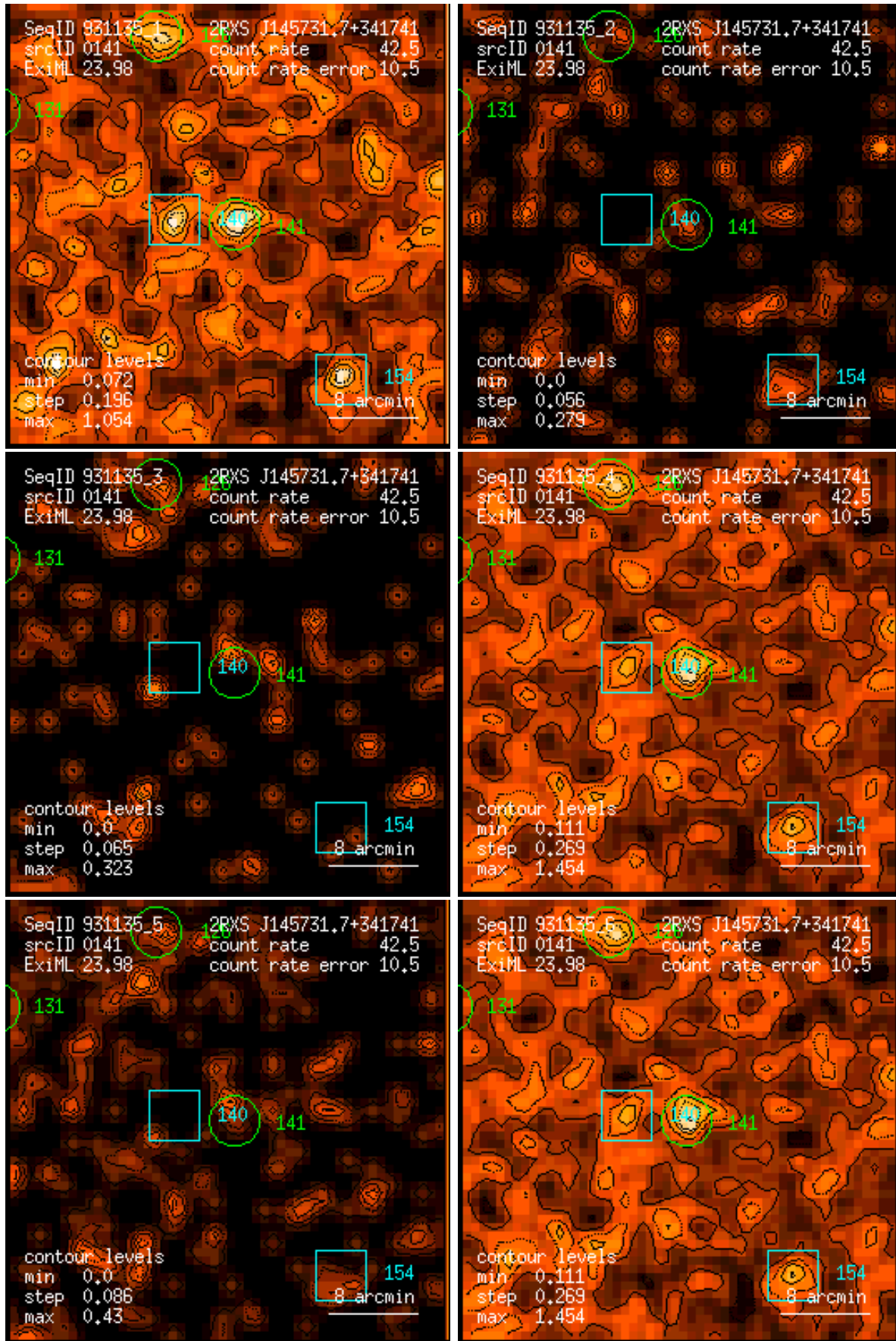
Figure 141: RASS 931135: detection 0141: band rate images, Gaussian filter: (1) PSPC channels 11 – 41, (2) 52 – 90, (3) 91 – 201, (4) 11 – 235, (5) 52 – 201, (6) 11 – 201. Broad band rates in counts/ks. Band rate contour levels in counts/ks/arcmin 2 .
