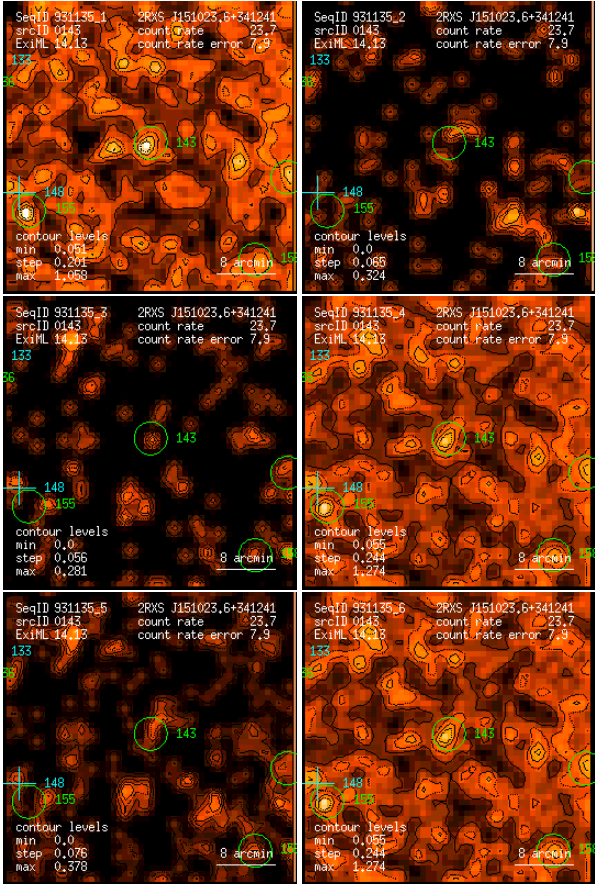
Figure 143: RASS 931135: detection 0143: band rate images, Gaussian filter: (1) PSPC channels 11 – 41, (2) 52 – 90, (3) 91 – 201, (4) 11 – 235, (5) 52 – 201, (6) 11 – 201. Broad band rates in counts/ks. Band rate contour levels in counts/ks/arcmin 2 .
