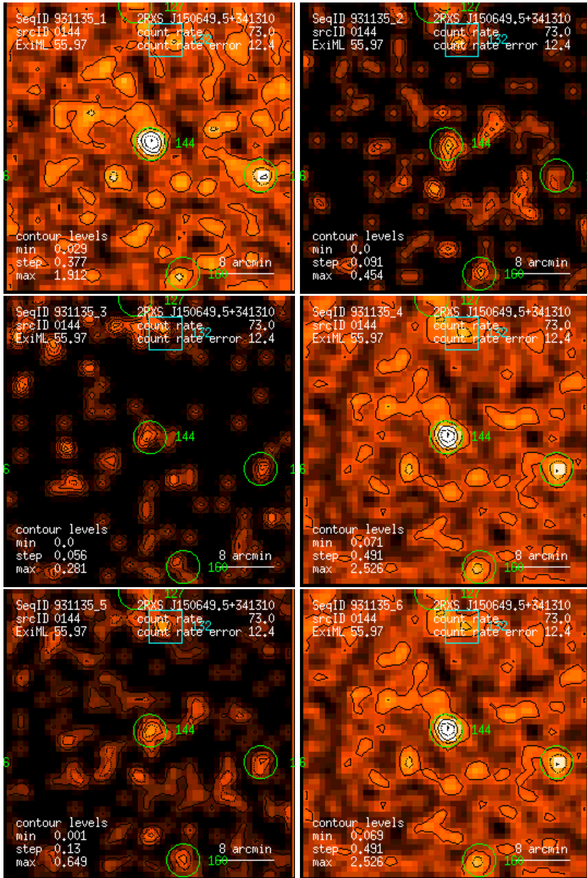
Figure 144: RASS 931135: detection 0144: band rate images, Gaussian filter: (1) PSPC channels 11 – 41, (2) 52 – 90, (3) 91 – 201, (4) 11 – 235, (5) 52 – 201, (6) 11 – 201. Broad band rates in counts/ks. Band rate contour levels in counts/ks/arcmin 2 .
