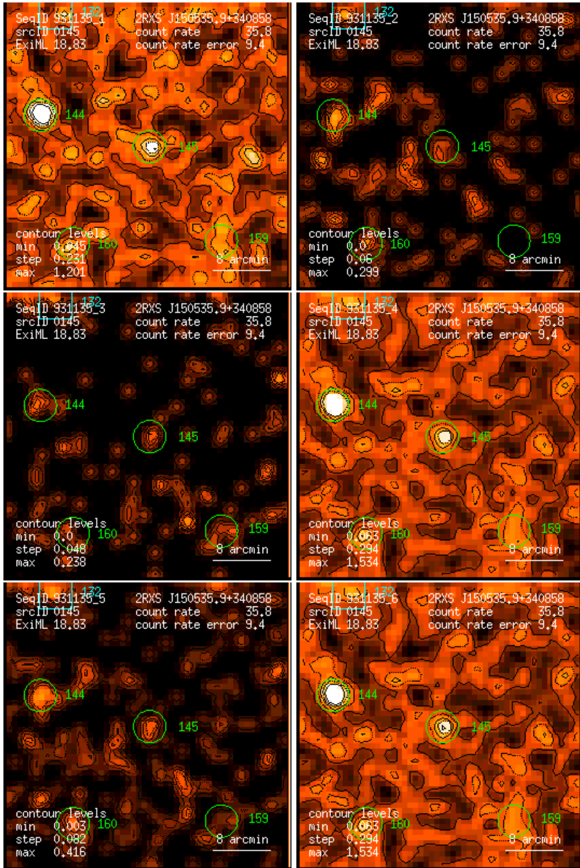
Figure 145: RASS 931135: detection 0145: band rate images, Gaussian filter: (1) PSPC channels 11 – 41, (2) 52 – 90, (3) 91 – 201, (4) 11 – 235, (5) 52 – 201, (6) 11 – 201. Broad band rates in counts/ks. Band rate contour levels in counts/ks/arcmin 2 .
