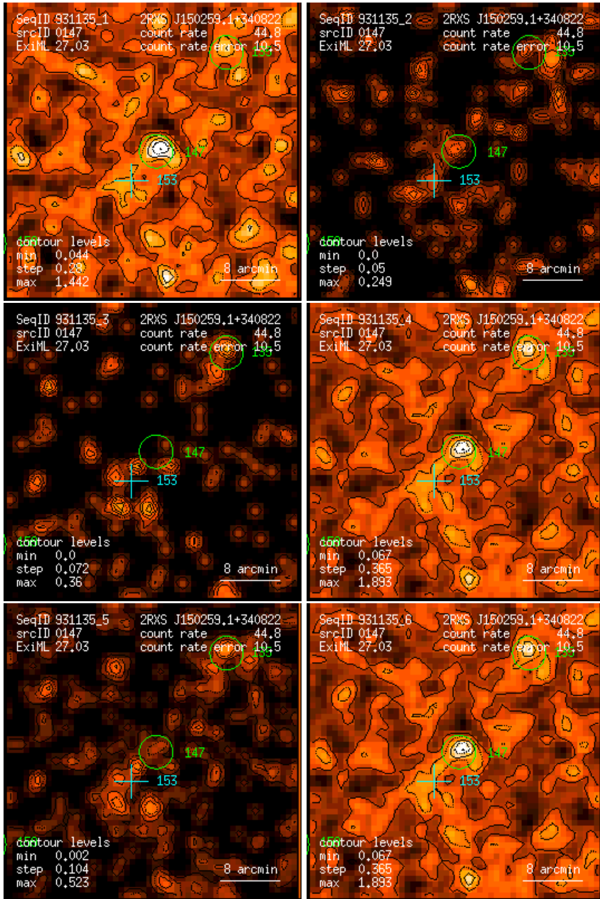
Figure 147: RASS 931135: detection 0147: band rate images, Gaussian filter: (1) PSPC channels 11 – 41, (2) 52 – 90, (3) 91 – 201, (4) 11 – 235, (5) 52 – 201, (6) 11 – 201. Broad band rates in counts/ks. Band rate contour levels in counts/ks/arcmin 2 .
