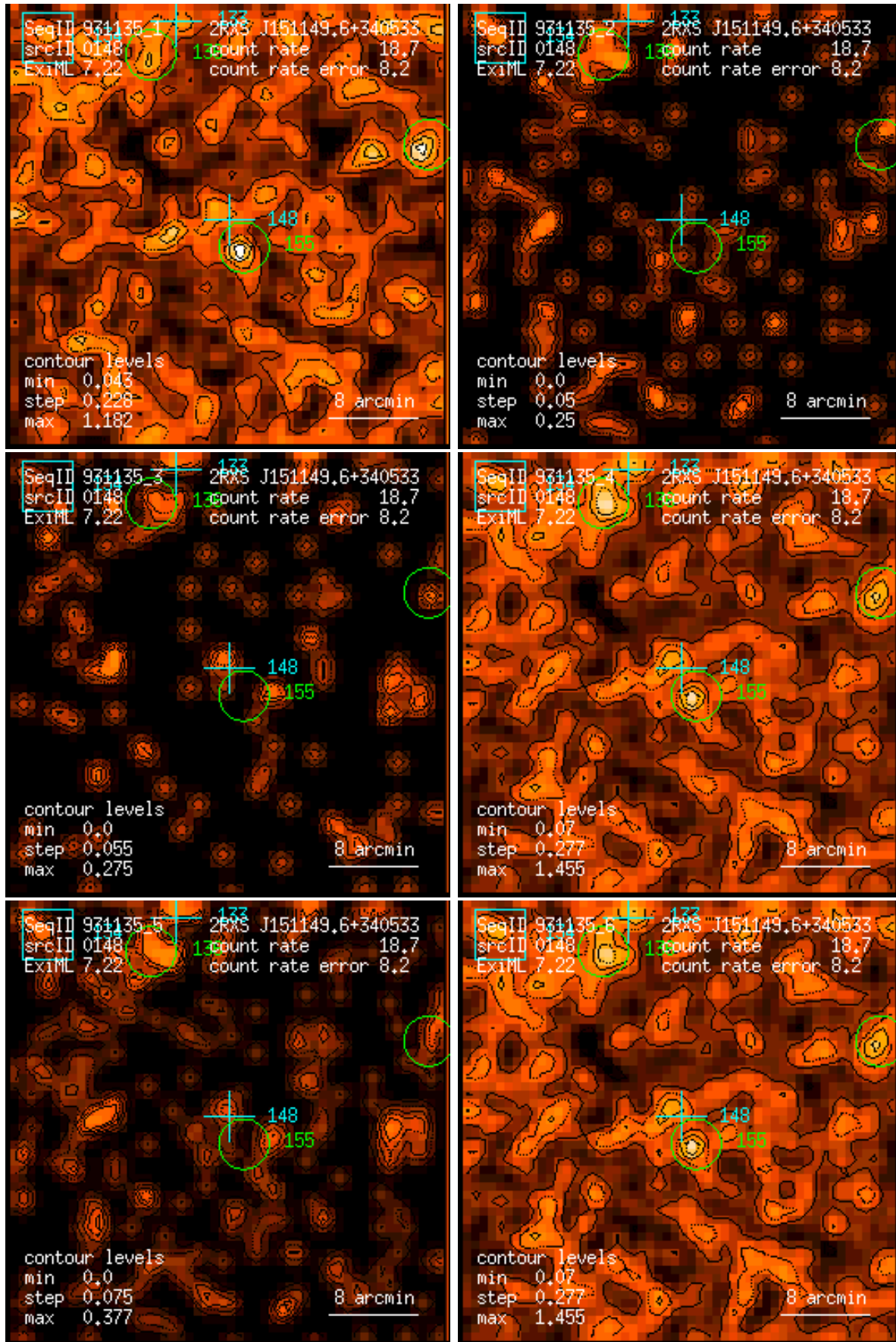
Figure 148: RASS 931135: detection 0148: band rate images, Gaussian filter: (1) PSPC channels 11 – 41, (2) 52 – 90, (3) 91 – 201, (4) 11 – 235, (5) 52 – 201, (6) 11 – 201. Broad band rates in counts/ks. Band rate contour levels in counts/ks/arcmin 2 .
