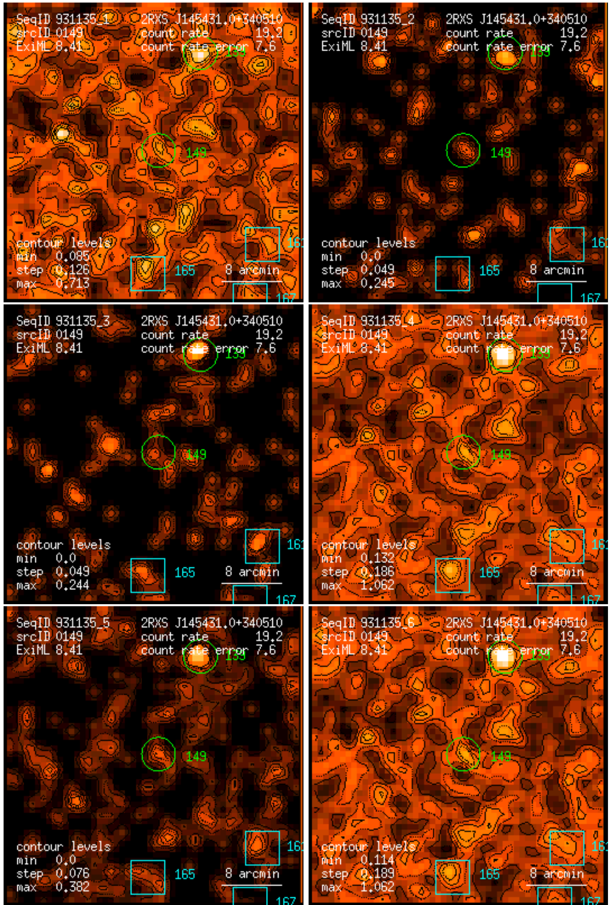
Figure 149: RASS 931135: detection 0149: band rate images, Gaussian filter: (1) PSPC channels 11 – 41, (2) 52 – 90, (3) 91 – 201, (4) 11 – 235, (5) 52 – 201, (6) 11 – 201. Broad band rates in counts/ks. Band rate contour levels in counts/ks/arcmin 2 .
