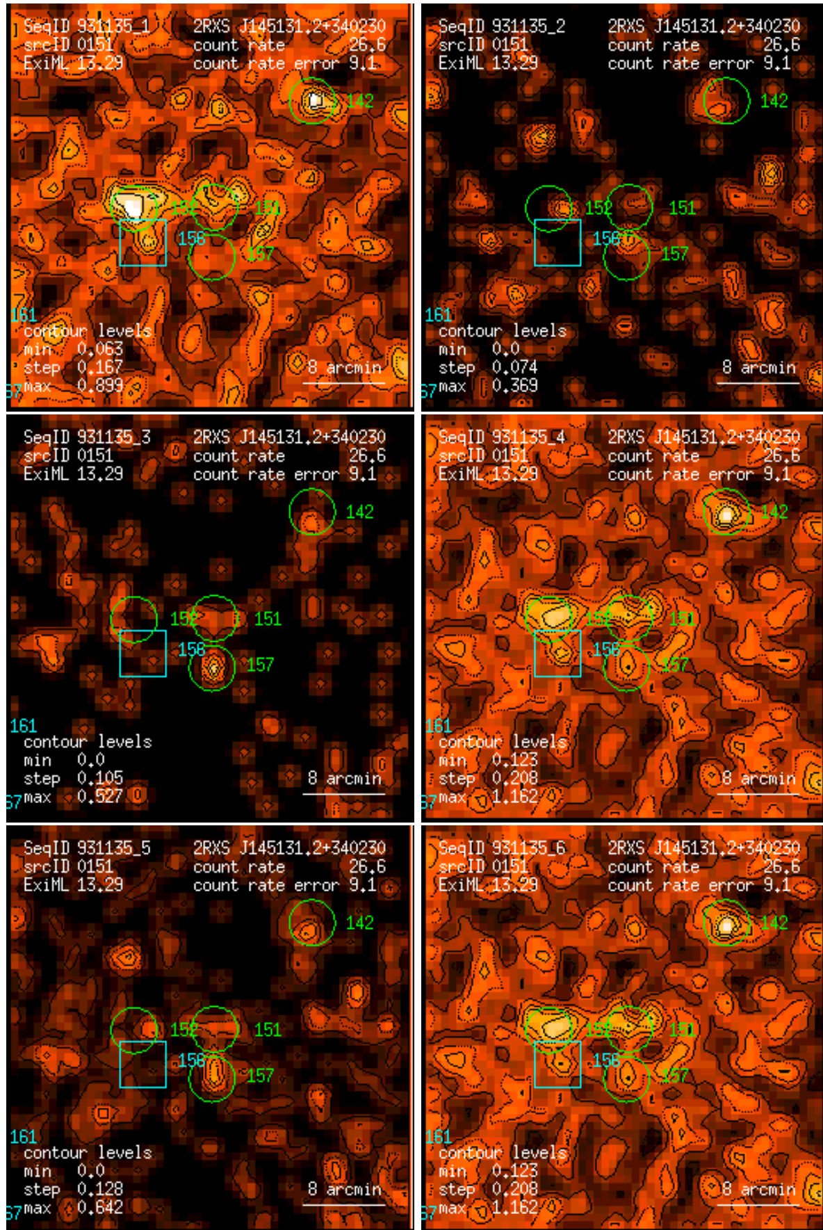
Figure 151: RASS 931135: detection 0151: band rate images, Gaussian filter: (1) PSPC channels 11 – 41, (2) 52 – 90, (3) 91 – 201, (4) 11 – 235, (5) 52 – 201, (6) 11 – 201. Broad band rates in counts/ks. Band rate contour levels in counts/ks/arcmin 2 .
