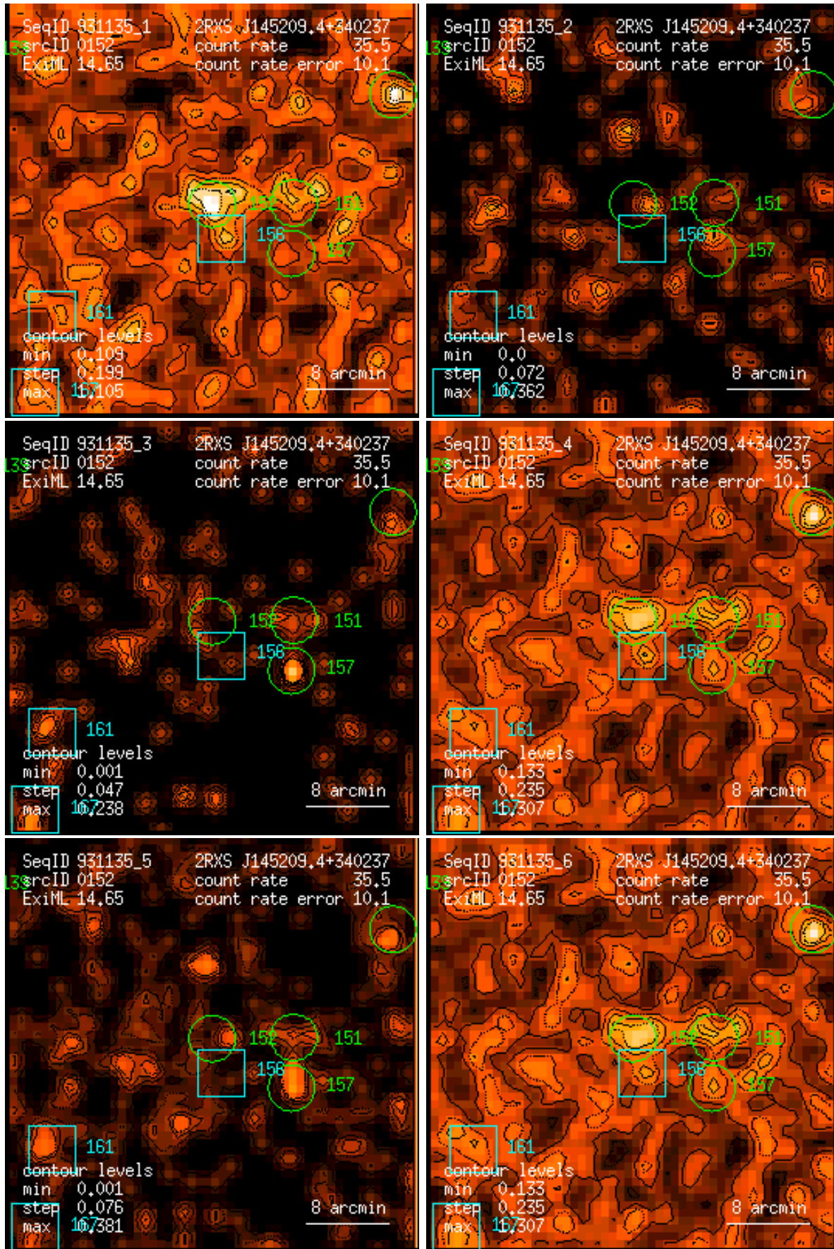
Figure 152: RASS 931135: detection 0152: band rate images, Gaussian filter: (1) PSPC channels 11 – 41, (2) 52 – 90, (3) 91 – 201, (4) 11 – 235, (5) 52 – 201, (6) 11 – 201. Broad band rates in counts/ks. Band rate contour levels in counts/ks/arcmin 2 .
