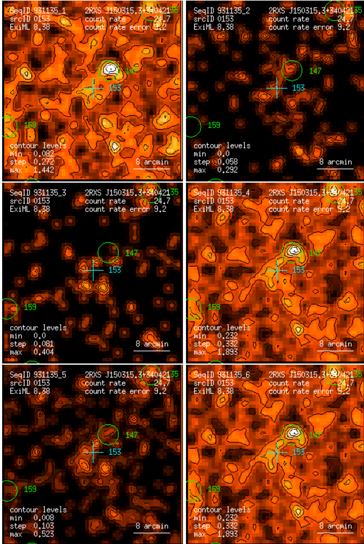
Figure 153: RASS 931135: detection 0153: band rate images, Gaussian filter: (1) PSPC channels 11 – 41, (2) 52 – 90, (3) 91 – 201, (4) 11 – 235, (5) 52 – 201, (6) 11 – 201. Broad band rates in counts/ks. Band rate contour levels in counts/ks/arcmin 2 .
