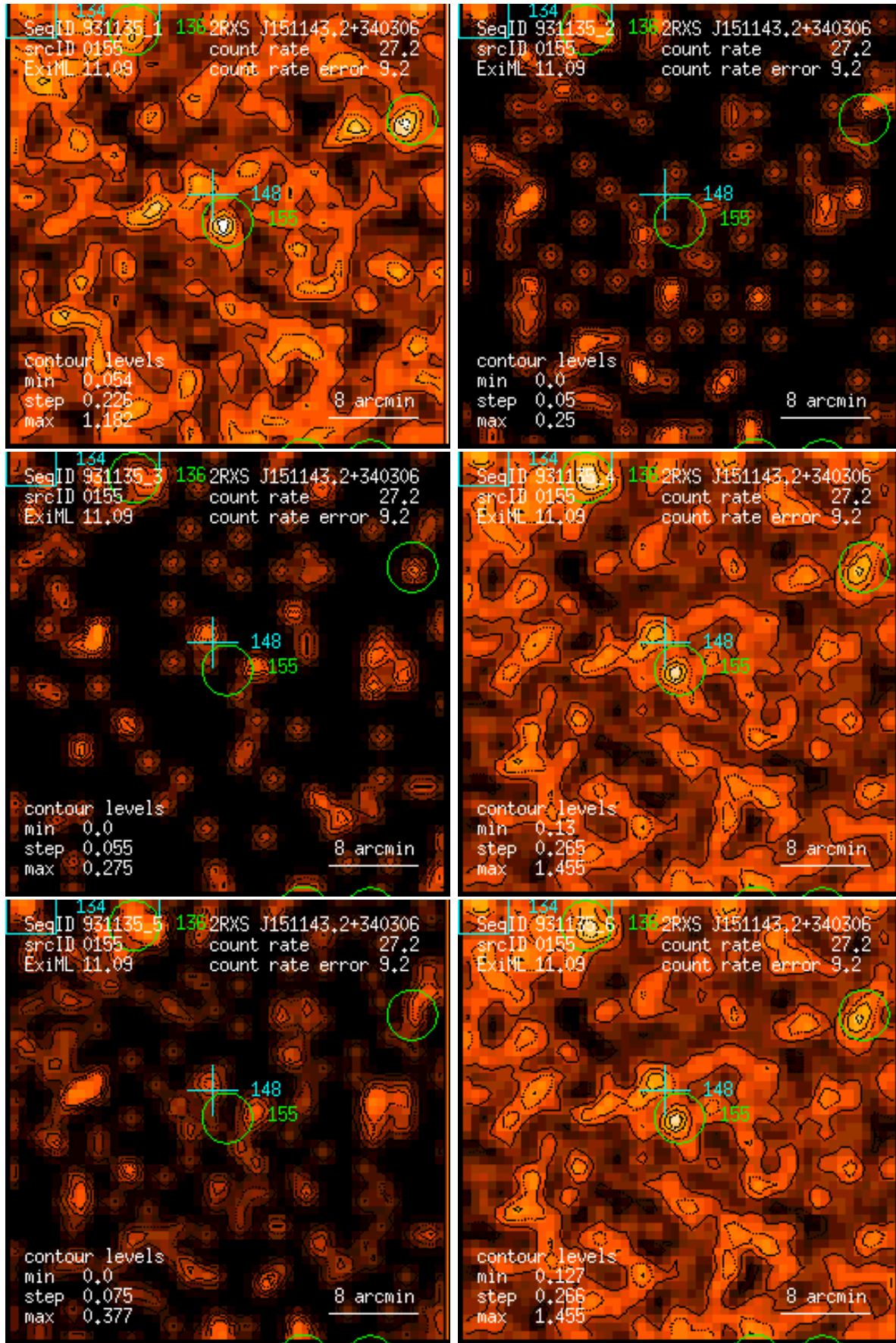
Figure 155: RASS 931135: detection 0155: band rate images, Gaussian filter: (1) PSPC channels 11 – 41, (2) 52 – 90, (3) 91 – 201, (4) 11 – 235, (5) 52 – 201, (6) 11 – 201. Broad band rates in counts/ks. Band rate contour levels in counts/ks/arcmin 2 .
