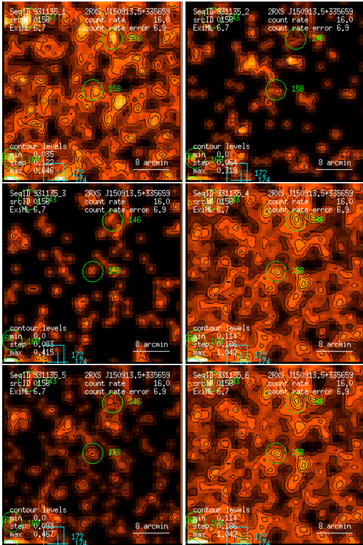
Figure 158: RASS 931135: detection 0158: band rate images, Gaussian filter: (1) PSPC channels 11 – 41, (2) 52 – 90, (3) 91 – 201, (4) 11 – 235, (5) 52 – 201, (6) 11 – 201. Broad band rates in counts/ks. Band rate contour levels in counts/ks/arcmin 2 .
