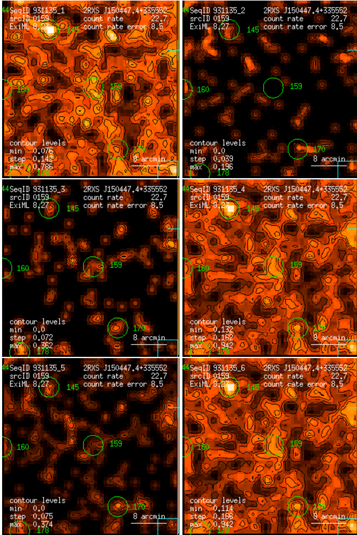
Figure 159: RASS 931135: detection 0159: band rate images, Gaussian filter: (1) PSPC channels 11 – 41, (2) 52 – 90, (3) 91 – 201, (4) 11 – 235, (5) 52 – 201, (6) 11 – 201. Broad band rates in counts/ks. Band rate contour levels in counts/ks/arcmin 2 .
