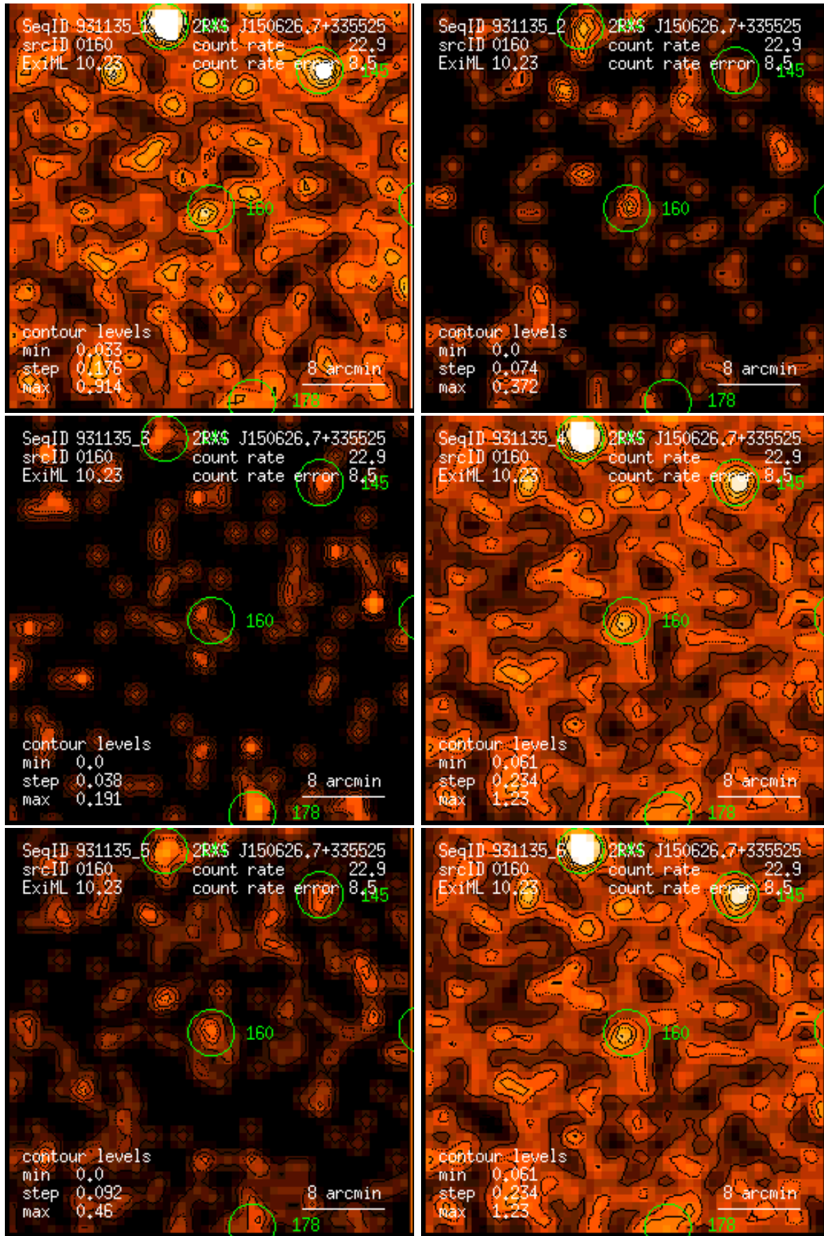
Figure 160: RASS 931135: detection 0160: band rate images, Gaussian filter: (1) PSPC channels 11 – 41, (2) 52 – 90, (3) 91 – 201, (4) 11 – 235, (5) 52 – 201, (6) 11 – 201. Broad band rates in counts/ks. Band rate contour levels in counts/ks/arcmin 2 .
