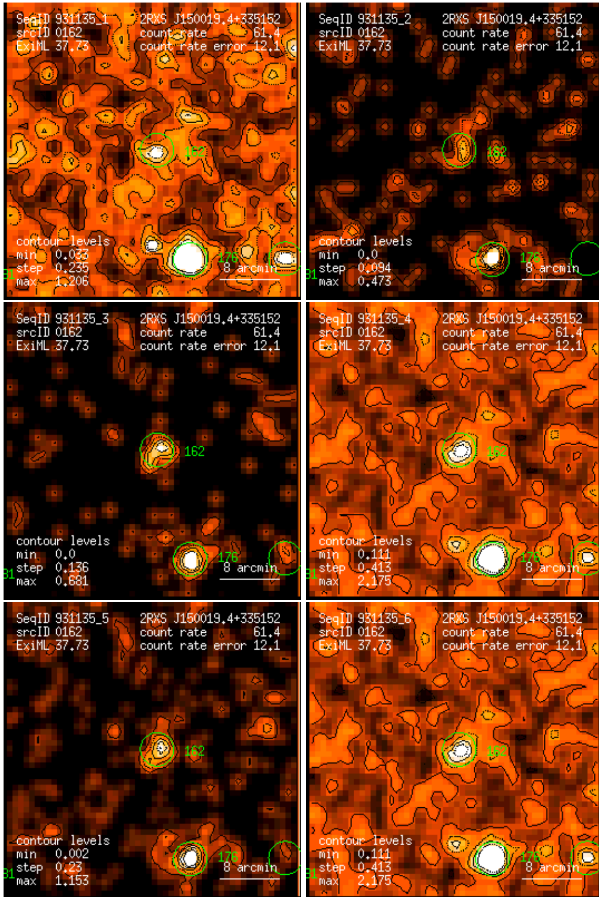
Figure 162: RASS 931135: detection 0162: band rate images, Gaussian filter: (1) PSPC channels 11 – 41, (2) 52 – 90, (3) 91 – 201, (4) 11 – 235, (5) 52 – 201, (6) 11 – 201. Broad band rates in counts/ks. Band rate contour levels in counts/ks/arcmin 2 .
