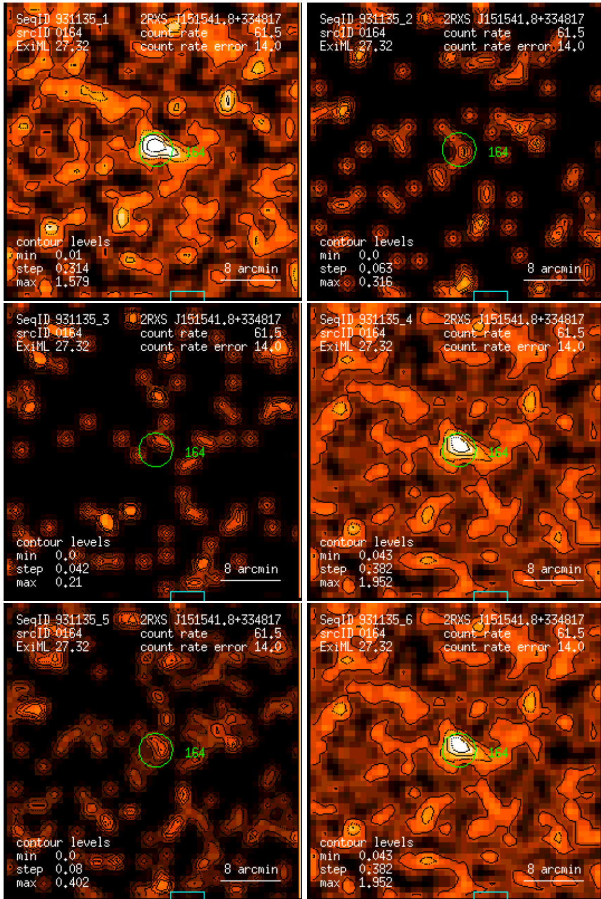
Figure 164: RASS 931135: detection 0164: band rate images, Gaussian filter: (1) PSPC channels 11 – 41, (2) 52 – 90, (3) 91 – 201, (4) 11 – 235, (5) 52 – 201, (6) 11 – 201. Broad band rates in counts/ks. Band rate contour levels in counts/ks/arcmin 2 .
