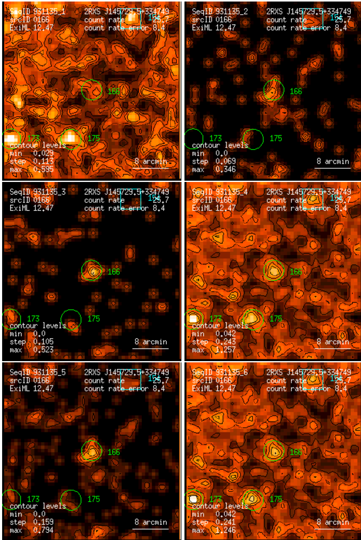
Figure 166: RASS 931135: detection 0166: band rate images, Gaussian filter: (1) PSPC channels 11 – 41, (2) 52 – 90, (3) 91 – 201, (4) 11 – 235, (5) 52 – 201, (6) 11 – 201. Broad band rates in counts/ks. Band rate contour levels in counts/ks/arcmin 2 .
