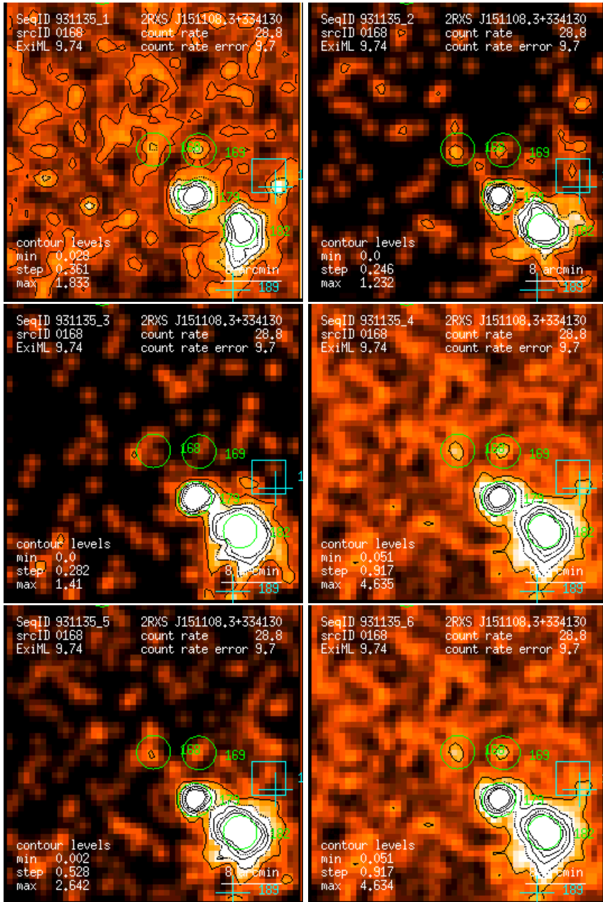
Figure 168: RASS 931135: detection 0168: band rate images, Gaussian filter: (1) PSPC channels 11 – 41, (2) 52 – 90, (3) 91 – 201, (4) 11 – 235, (5) 52 – 201, (6) 11 – 201. Broad band rates in counts/ks. Band rate contour levels in counts/ks/arcmin 2 .
