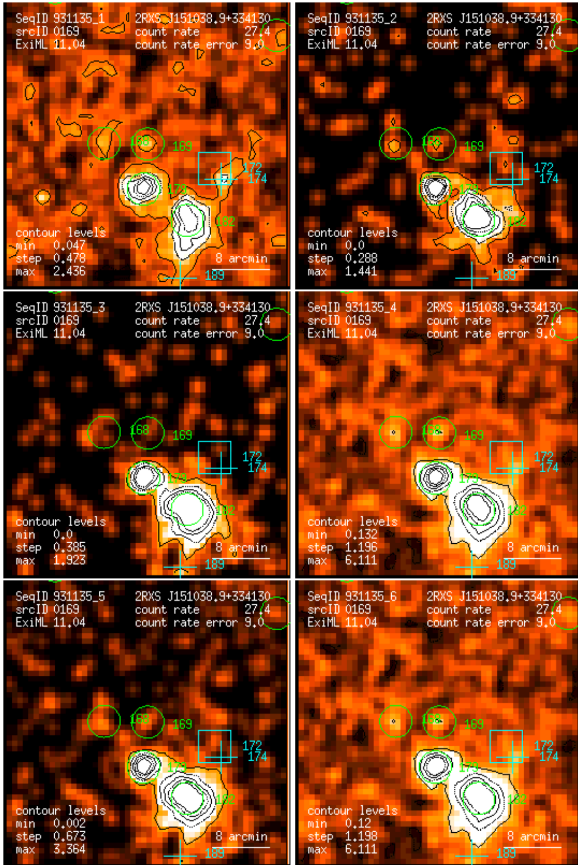
Figure 169: RASS 931135: detection 0169: band rate images, Gaussian filter: (1) PSPC channels 11 – 41, (2) 52 – 90, (3) 91 – 201, (4) 11 – 235, (5) 52 – 201, (6) 11 – 201. Broad band rates in counts/ks. Band rate contour levels in counts/ks/arcmin 2 .
