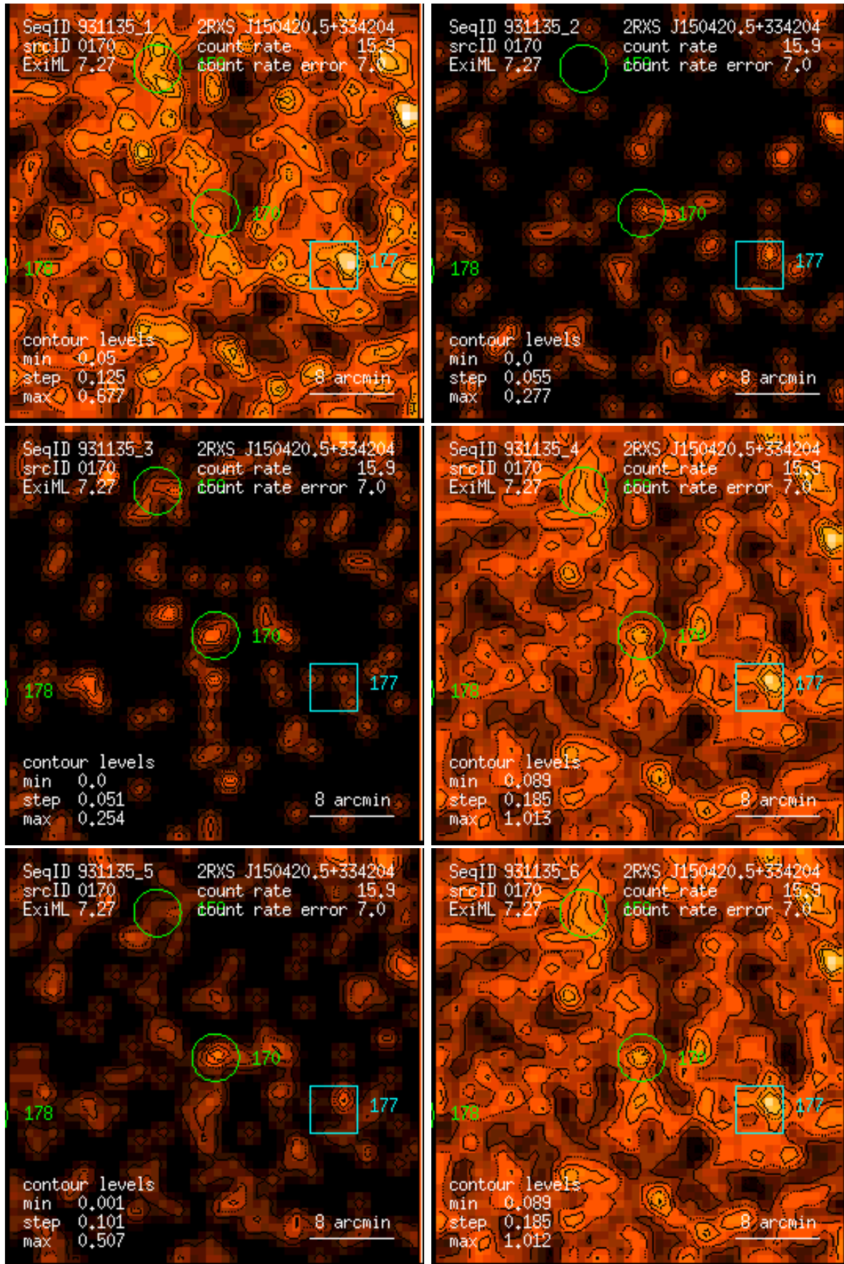
Figure 170: RASS 931135: detection 0170: band rate images, Gaussian filter: (1) PSPC channels 11 – 41, (2) 52 – 90, (3) 91 – 201, (4) 11 – 235, (5) 52 – 201, (6) 11 – 201. Broad band rates in counts/ks. Band rate contour levels in counts/ks/arcmin 2 .
