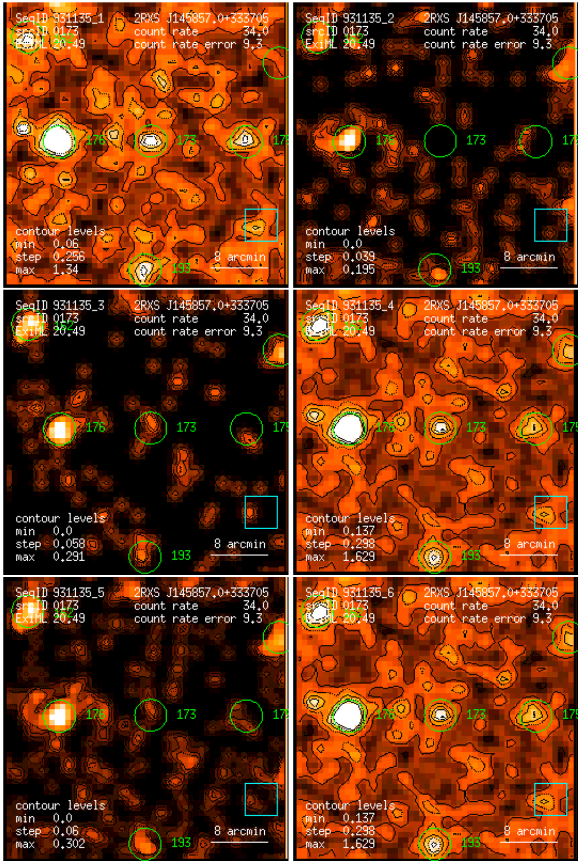
Figure 173: RASS 931135: detection 0173: band rate images, Gaussian filter: (1) PSPC channels 11 – 41, (2) 52 – 90, (3) 91 – 201, (4) 11 – 235, (5) 52 – 201, (6) 11 – 201. Broad band rates in counts/ks. Band rate contour levels in counts/ks/arcmin 2 .
