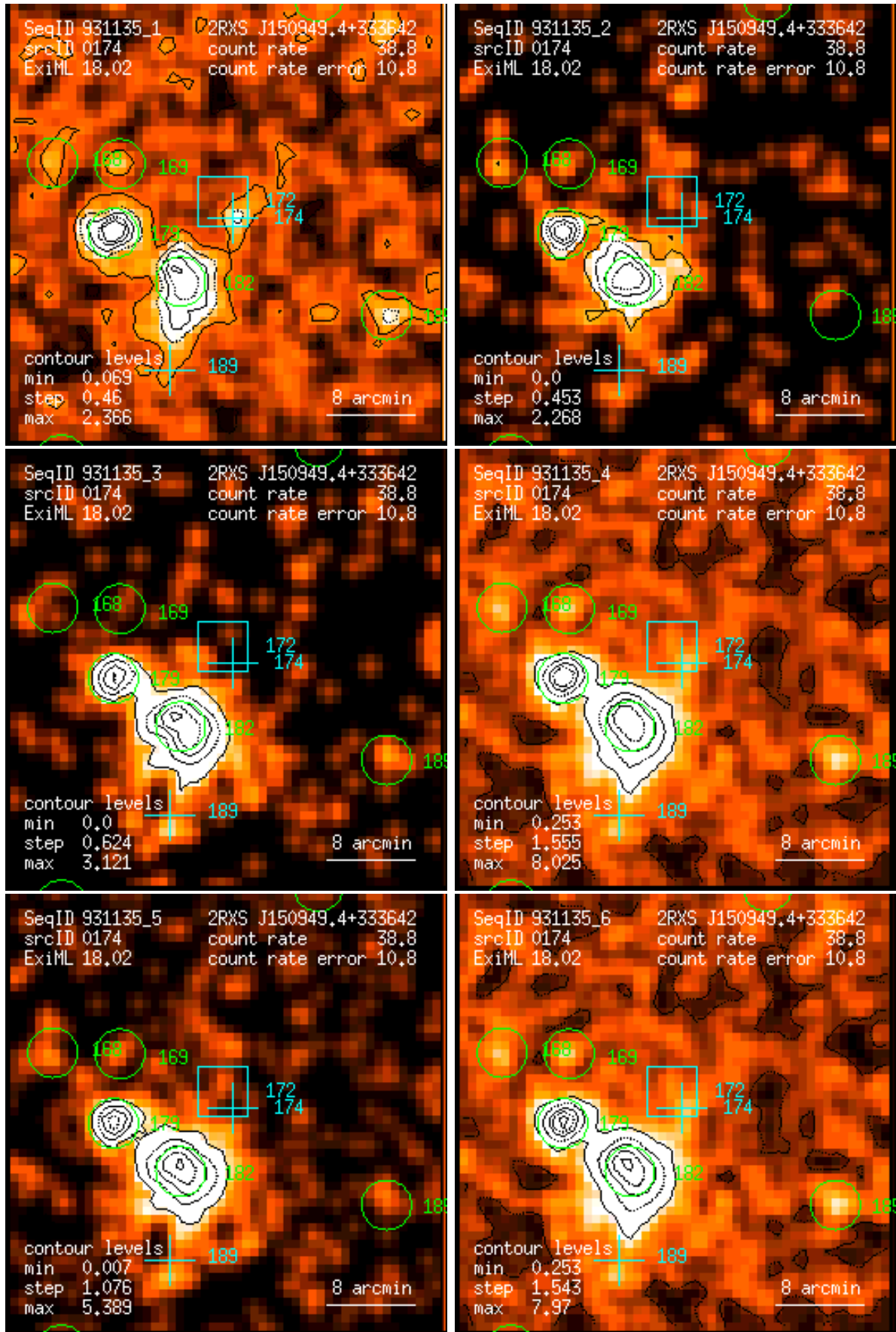
Figure 174: RASS 931135: detection 0174: band rate images, Gaussian filter: (1) PSPC channels 11 – 41, (2) 52 – 90, (3) 91 – 201, (4) 11 – 235, (5) 52 – 201, (6) 11 – 201. Broad band rates in counts/ks. Band rate contour levels in counts/ks/arcmin 2 .
