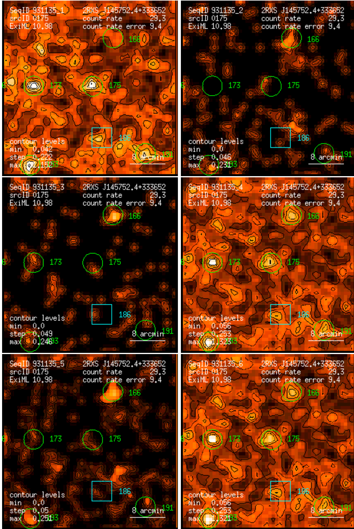
Figure 175: RASS 931135: detection 0175: band rate images, Gaussian filter: (1) PSPC channels 11 – 41, (2) 52 – 90, (3) 91 – 201, (4) 11 – 235, (5) 52 – 201, (6) 11 – 201. Broad band rates in counts/ks. Band rate contour levels in counts/ks/arcmin 2 .
