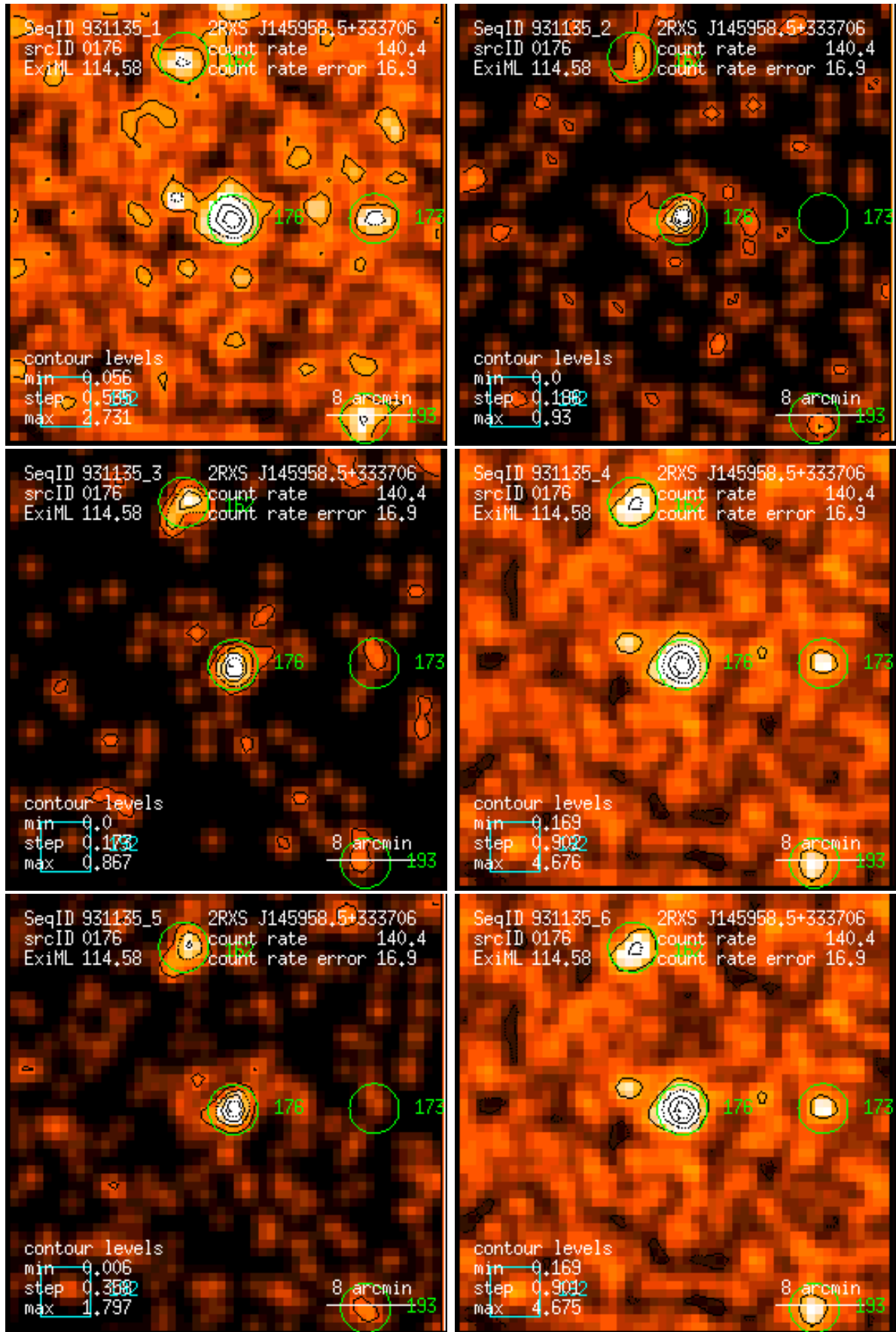
Figure 176: RASS 931135: detection 0176: band rate images, Gaussian filter: (1) PSPC channels 11 – 41, (2) 52 – 90, (3) 91 – 201, (4) 11 – 235, (5) 52 – 201, (6) 11 – 201. Broad band rates in counts/ks. Band rate contour levels in counts/ks/arcmin 2 .
