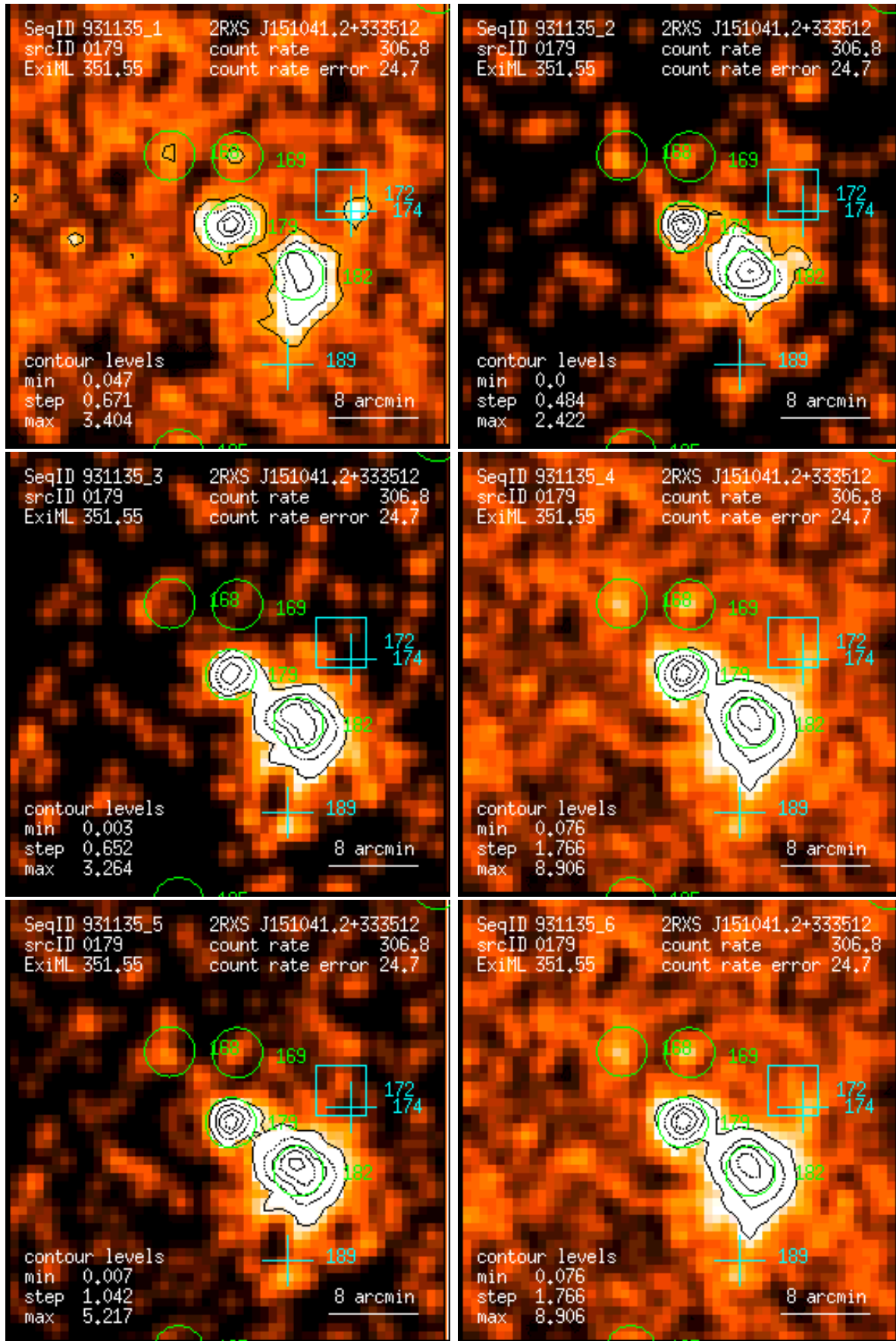
Figure 179: RASS 931135: detection 0179: band rate images, Gaussian filter: (1) PSPC channels 11 – 41, (2) 52 – 90, (3) 91 – 201, (4) 11 – 235, (5) 52 – 201, (6) 11 – 201. Broad band rates in counts/ks. Band rate contour levels in counts/ks/arcmin 2 .
