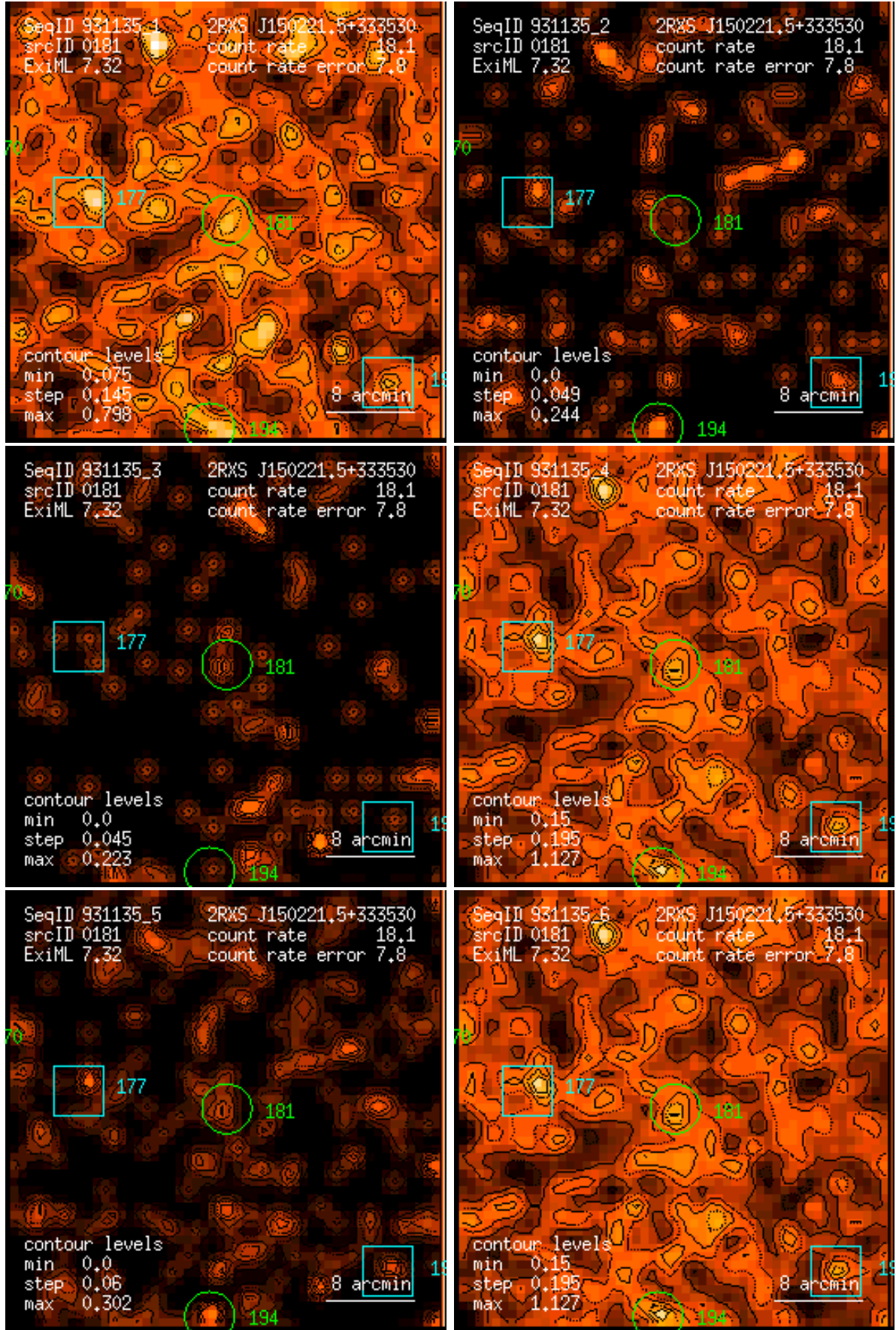
Figure 181: RASS 931135: detection 0181: band rate images, Gaussian filter: (1) PSPC channels 11 – 41, (2) 52 – 90, (3) 91 – 201, (4) 11 – 235, (5) 52 – 201, (6) 11 – 201. Broad band rates in counts/ks. Band rate contour levels in counts/ks/arcmin 2 .
