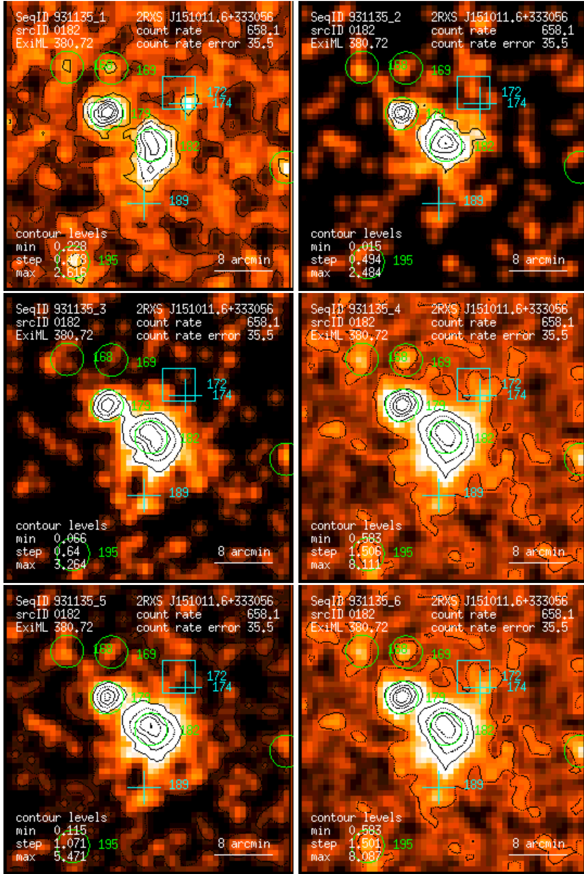
Figure 182: RASS 931135: detection 0182: band rate images, Gaussian filter: (1) PSPC channels 11 – 41, (2) 52 – 90, (3) 91 – 201, (4) 11 – 235, (5) 52 – 201, (6) 11 – 201. Broad band rates in counts/ks. Band rate contour levels in counts/ks/arcmin 2 .
