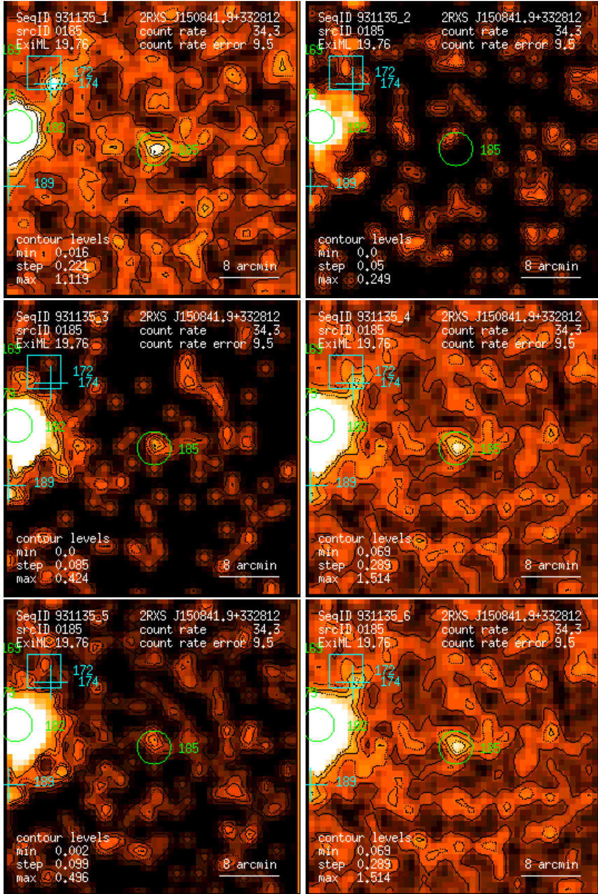
Figure 185: RASS 931135: detection 0185: band rate images, Gaussian filter: (1) PSPC channels 11 – 41, (2) 52 – 90, (3) 91 – 201, (4) 11 – 235, (5) 52 – 201, (6) 11 – 201. Broad band rates in counts/ks. Band rate contour levels in counts/ks/arcmin 2 .
